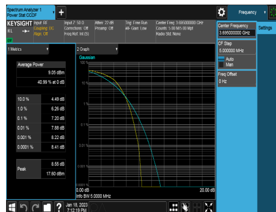
Ant 2_10M_QPSK_FULLRB_PAPR_Middle channel
