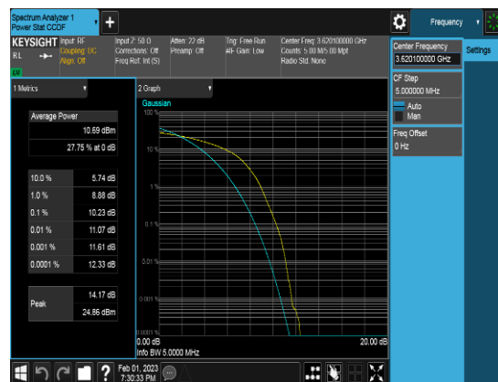
PCC_20M_3620.1MHz_QPSK_FULLRB_PAPR
