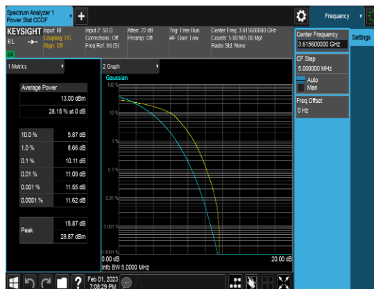
PCC_10M_3615.6MHz_Q64_FULLRB_PAPR
