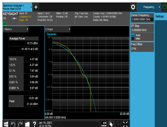
Ant 2_20M_Q64_1RB0_PAPR_Middle channel
