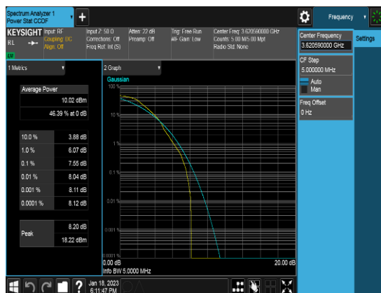
Ant 2_10M_QPSK_FULLRB_PAPR_Low channel
