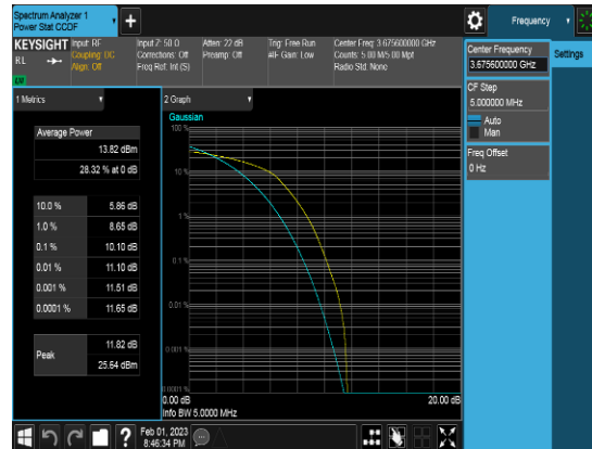
PCC_10M_3675.6MHz_Q64_FULLRB_PAPR
