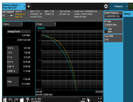
Ant 2_20M_Q16_FULLRB_PAPR_Low channel
