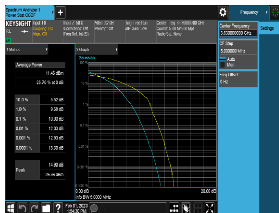
SCC_20M_3630MHz_QPSK_FULLRB_PAPR
