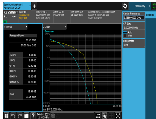
SCC_20M_3569.9MHz_QPSK_FULLRB_PAPR
