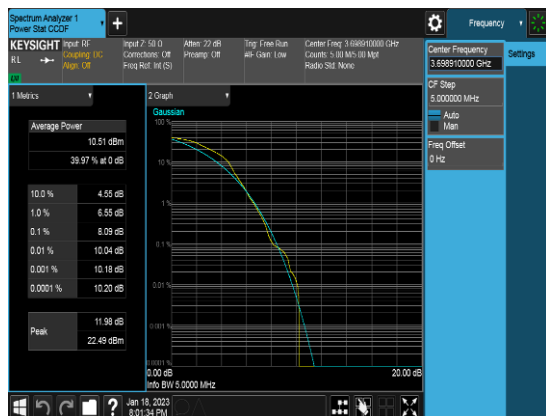
Ant 2_20M_Q16_1RB0_PAPR_Middle channel
