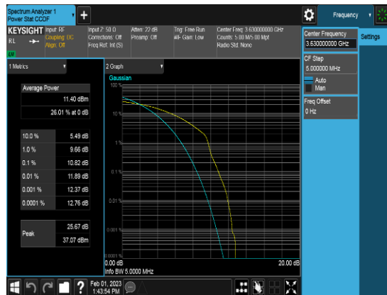
SCC_20M_3630MHz_Q64_FULLRB_PAPR
