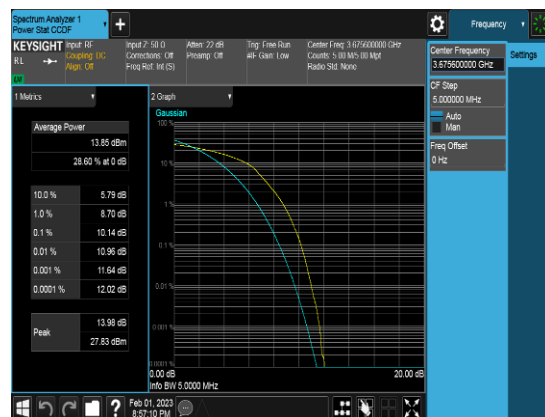
PCC_10M_3675.6MHz_QPSK_FULLRB_PAPR
