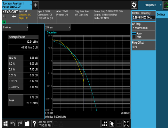
Ant 2_20M_QPSK_1RB0_PAPR_Middle channel
