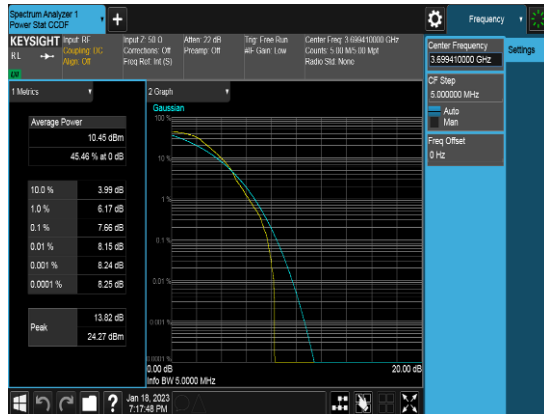
Ant 2_10M_QPSK_1RB0_PAPR_Middle channel
