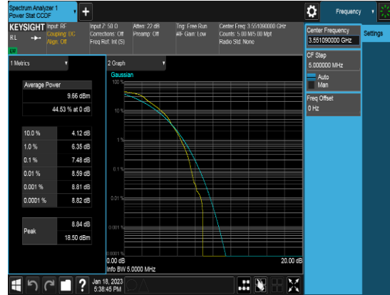
Ant 2_20M_QPSK_FULLRB_PAPR_High channel
