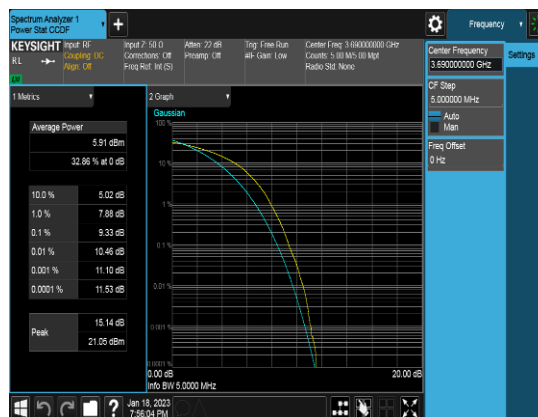
Ant 2_20M_Q16_FULLRB_PAPR_Middle channel
