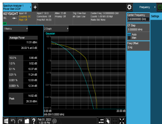
SCC_20M_3630MHz_QPSK_FULLRB_PAPR
