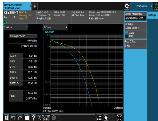
PCC_20M_3620.1MHz_Q64_FULLRB_PAPR
