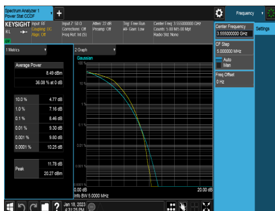
Ant 2_10M_Q64_FULLLRB_PAPR_Low channel
