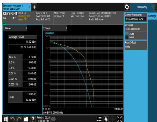
SCC_20M_3690MHz_QPSK_FULLRB_PAPR
