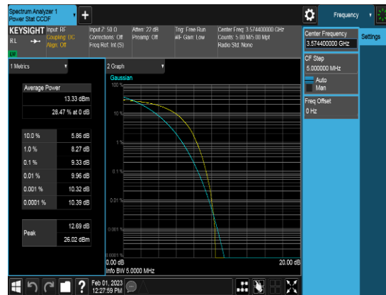
SCC_10M_3574.4MHz_QPSK_FULLRB_PAPR
