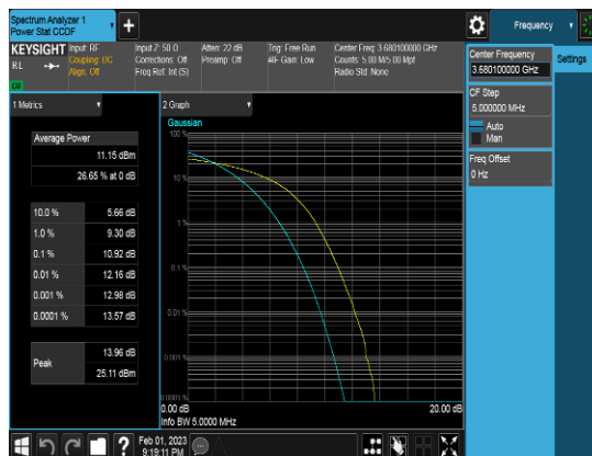
PCC_20M_3680.1MHz_Q64_FULLRB_PAPR
