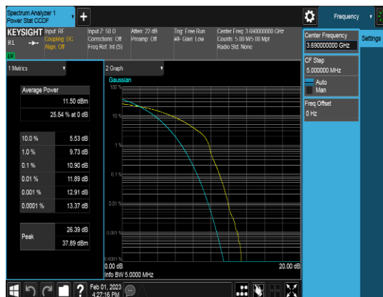
SCC_20M_3690MHz_Q64_FULLRB_PAPR
