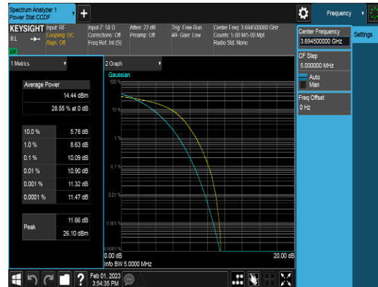
SCC_10M_3694.5MHz_Q64_FULLRB_PAPR
