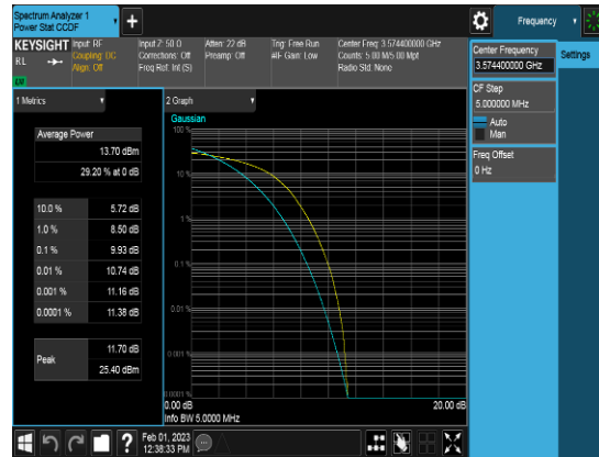
SCC_10M_3574.4MHz_Q64_FULLRB_PAPR
