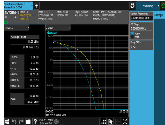
PCC_20M_3670.2MHz_Q64_FULLRB_PAPR
