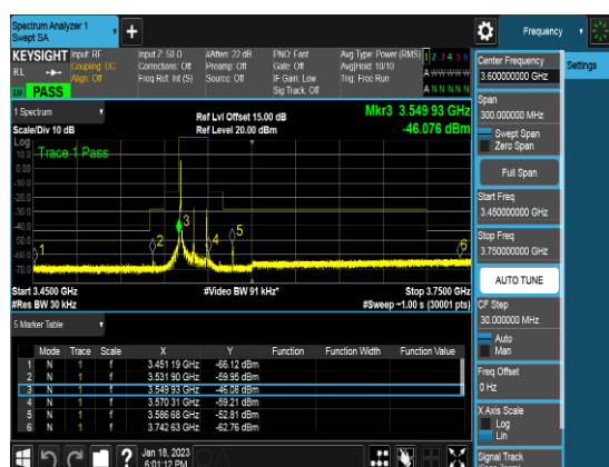
Ant 2_20M_Q64_1RB0_CSEpart96_Low channel
