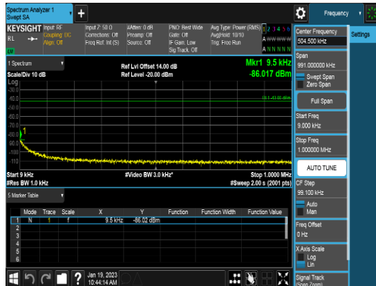
Ant 2_20M_Q64_1RB0_CSE0a_Middle channel
