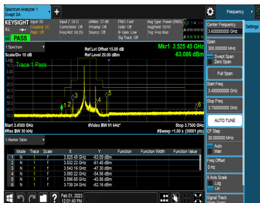
SCC_20M_3569.9MHz_QPSK_1RB_CSEpart96
