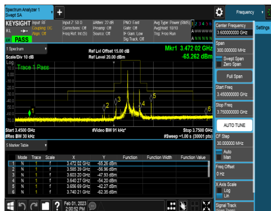
SCC_20M_3630MHz_Q64_1RB_CSEpart96
