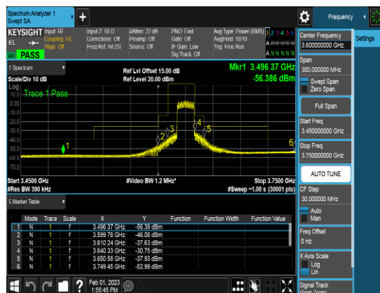
SCC_20M_3630MHz_Q64_FULLLRB_CSEpart96
