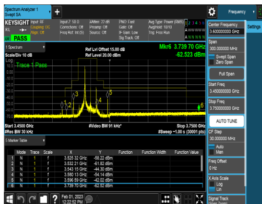
SCC_20M_3569.9MHz_Q64_1RB_CSEpart96
