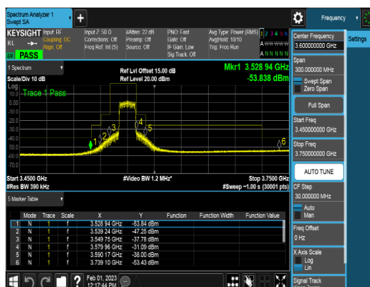
SCC_20M_3569.9MHz_Q64_FULLLRB_CSEpart9 6
