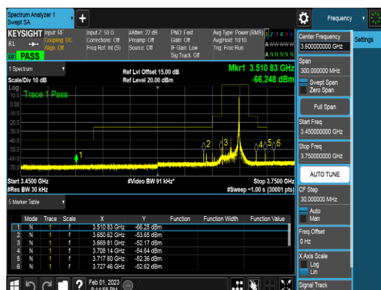
PCC_20M_3680.1MHz_QPSK_1RB_CSEpart96
