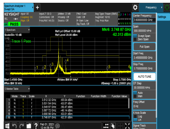
SCC_10M_3574.4MHz_Q16_1RB_CSEpart96
