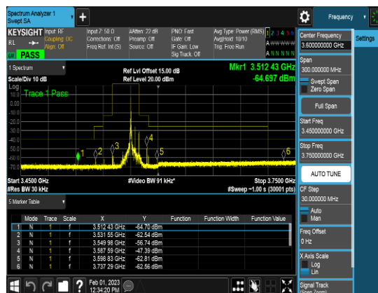
SCC_10M_3574.4MHz_QPSK_1RB_CSEpart96
