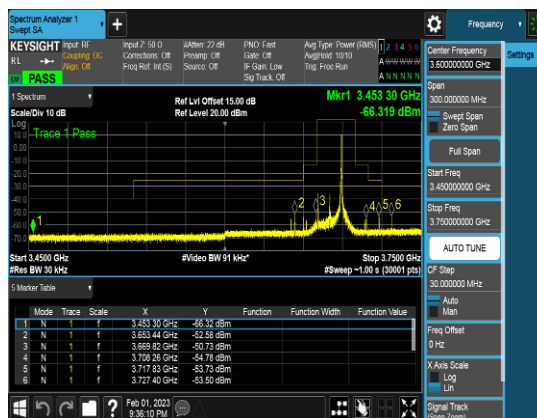
PCC_20M_3680.1MHz_Q64_1RB_CSEpart96
