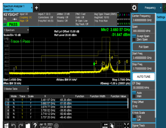
20M_Q16_1RB0_CSEpart96_Middle Channel
