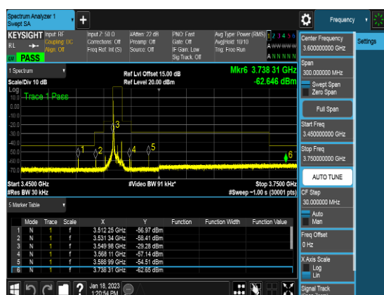
Ant 0_10M_Q64_1RB0_CSEpart96_Low channel
