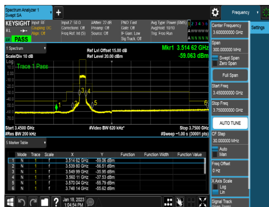
Ant 0_10M_Q16_FULLRB_CSEpart96_Low channel
