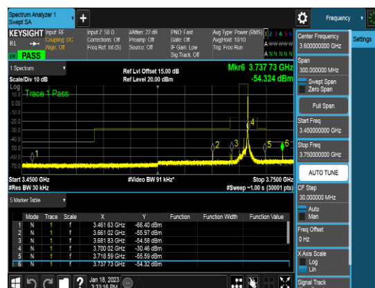
Ant 0_10M_Q64_1RB0_CSEpart96_Middle channel
