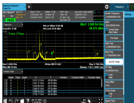
Ant 0_10M_Q16_1RB0_CSEpart96_Low channel
