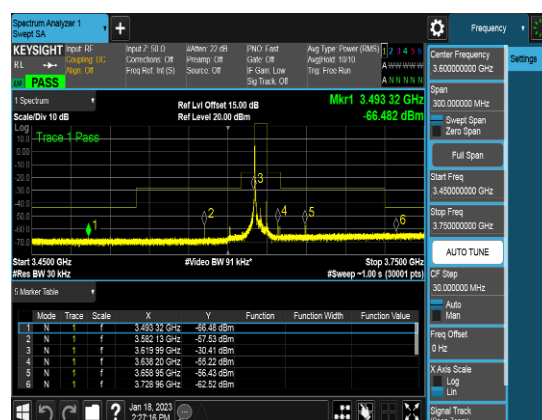
Ant 0_10M_Q64_1RB0_CSEpart96_Middle channel
