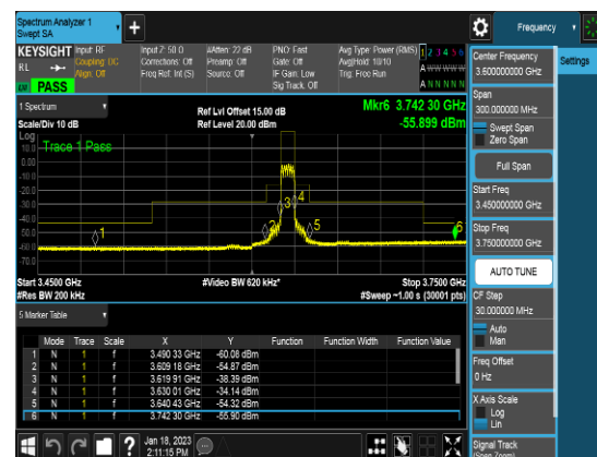
Ant 0_10M_Q16_FULLRB_CSEpart96_Middle channel
