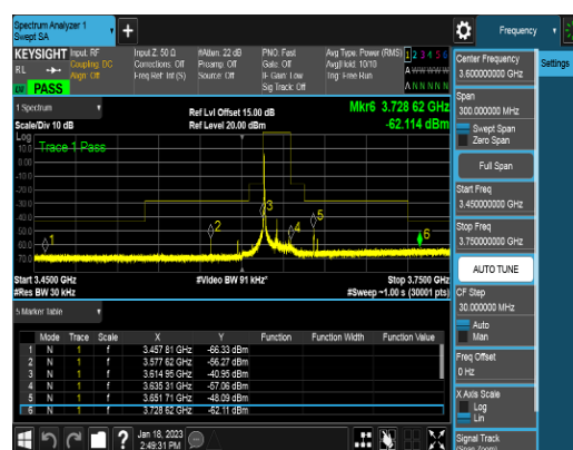
Ant 0_20M_Q16_1RB0_CSEpart96_Middle channel
