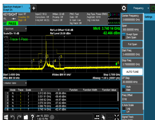
Ant 0_20M_Q16_1RB0_CSEpart96_Low channel
