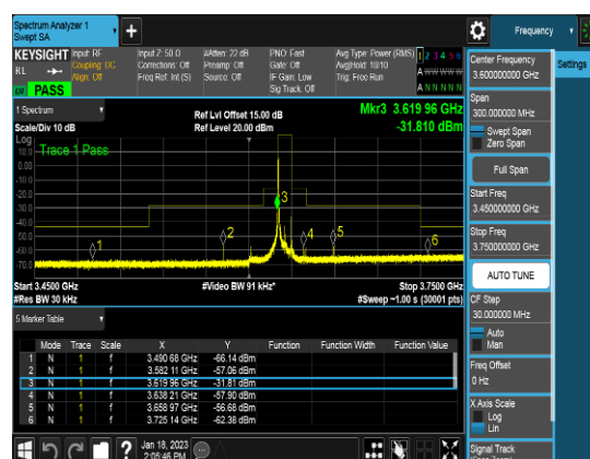
Ant 0_10M_QPSK_1RB0_CSEpart96_Middle channel
