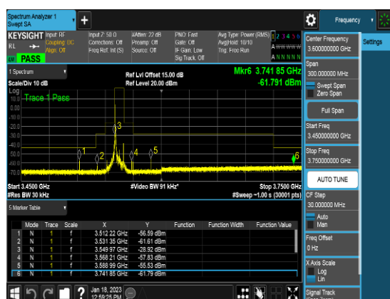
Ant 0_10M_QPSK_1RB0_CSEpart96_Low channel
