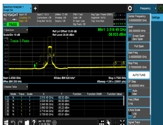
Ant 0_10M_Q64_FULLRB_CSEpart96_Low channel
