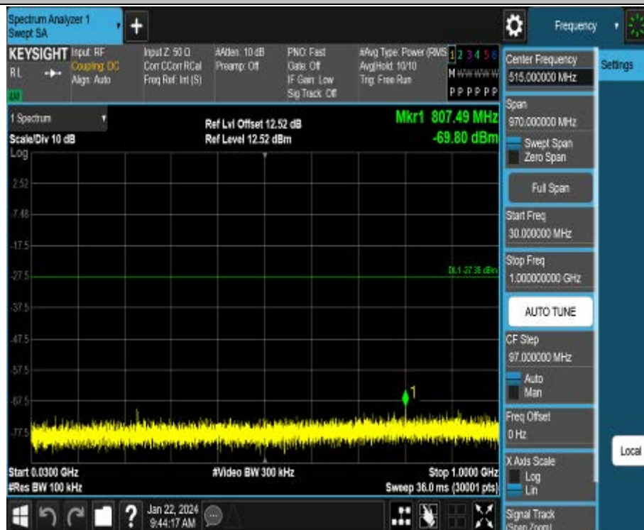
11B-CDD_Ant1_2437_30~1000
