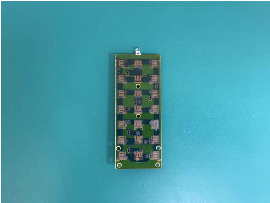
Internal: Top
