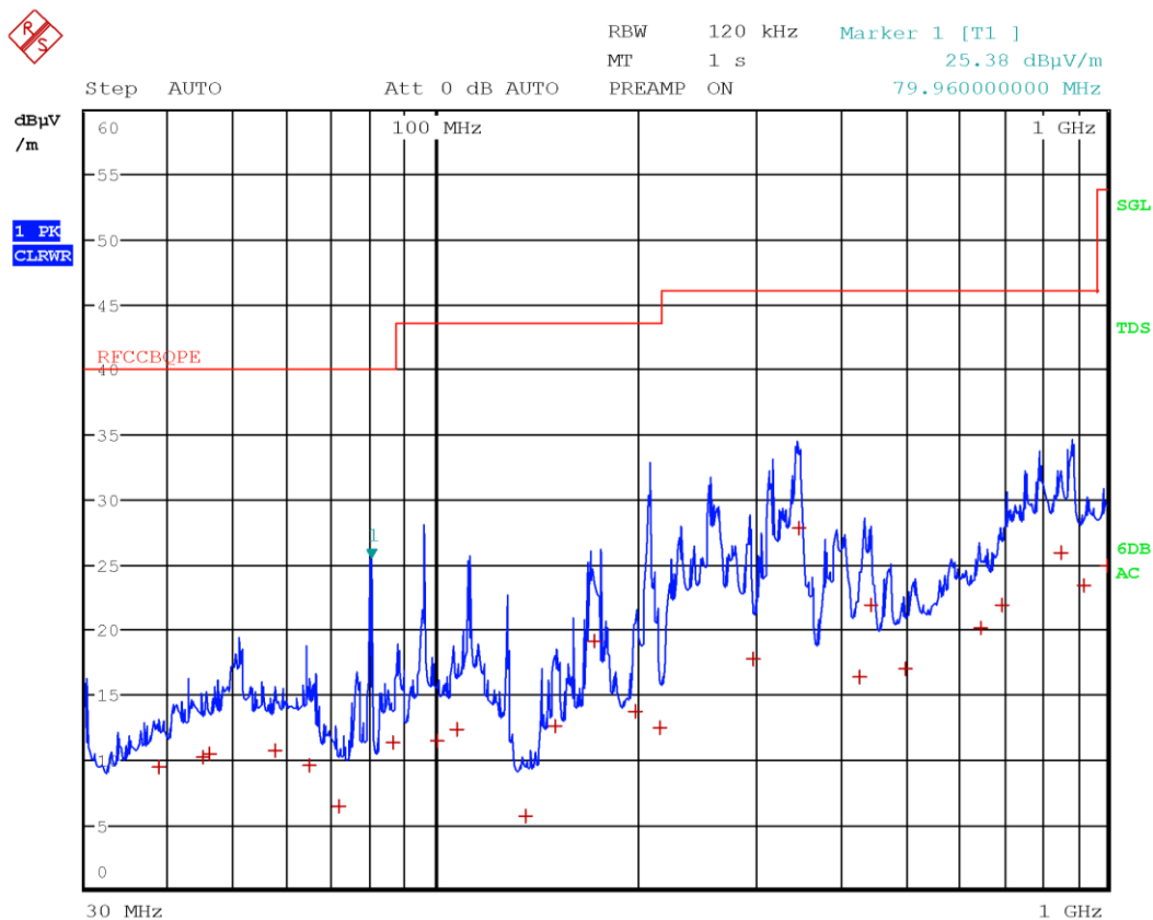
Figure 8.3-2: Radiated emissions with antenna in horizontal polarization (30 - 1000 MHz)
