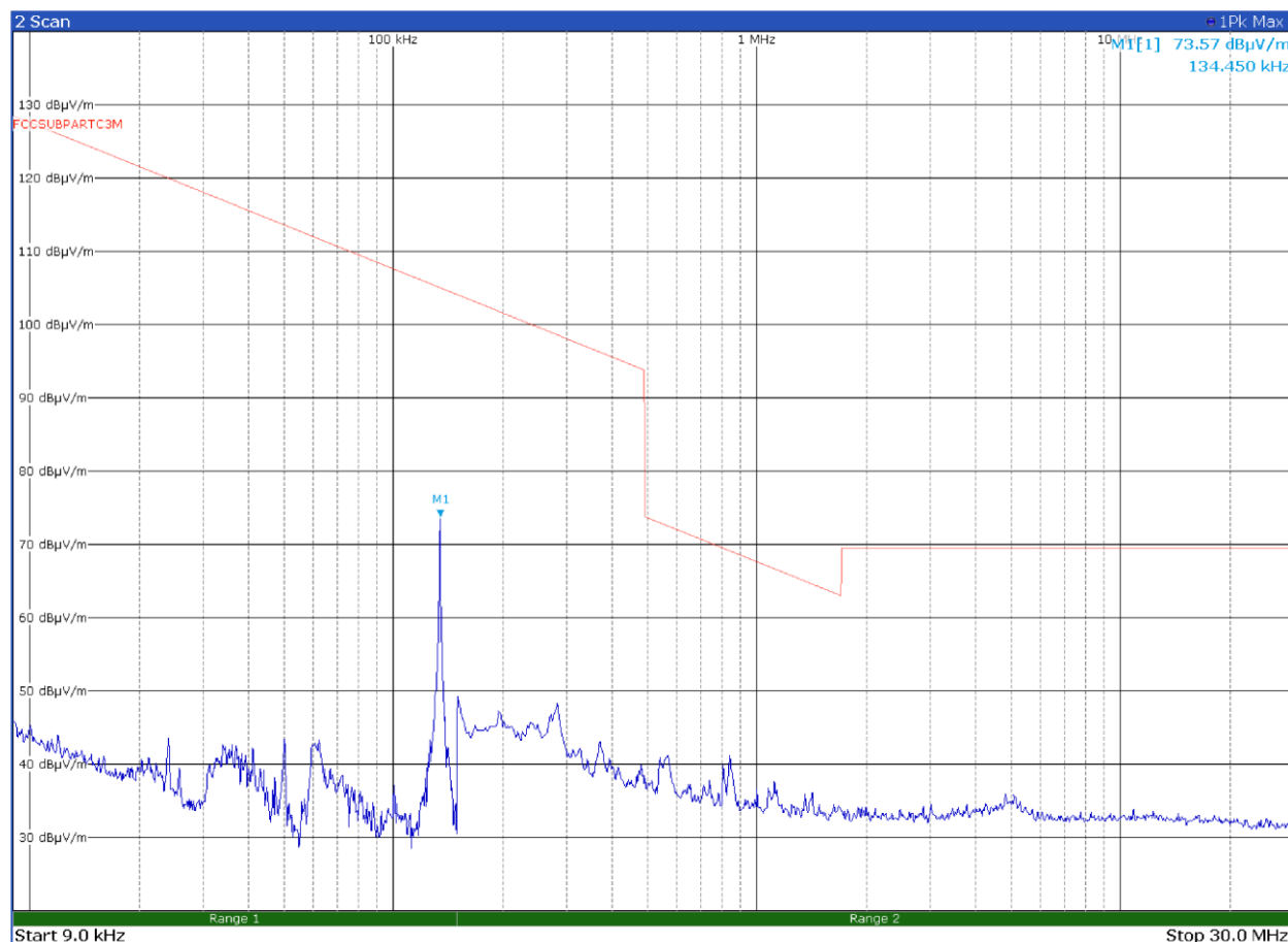
Figure 8.3-1: Radiated emissions with antenna loop (9 kHz – 30 MHz)
