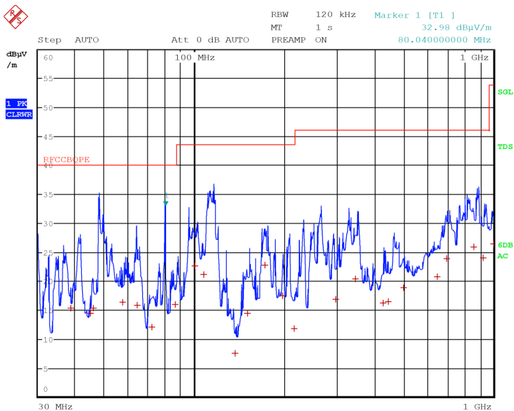
Figure 8.3-3: Radiated emissions with antenna in vertical polarization (30 - 1000 MHz)
