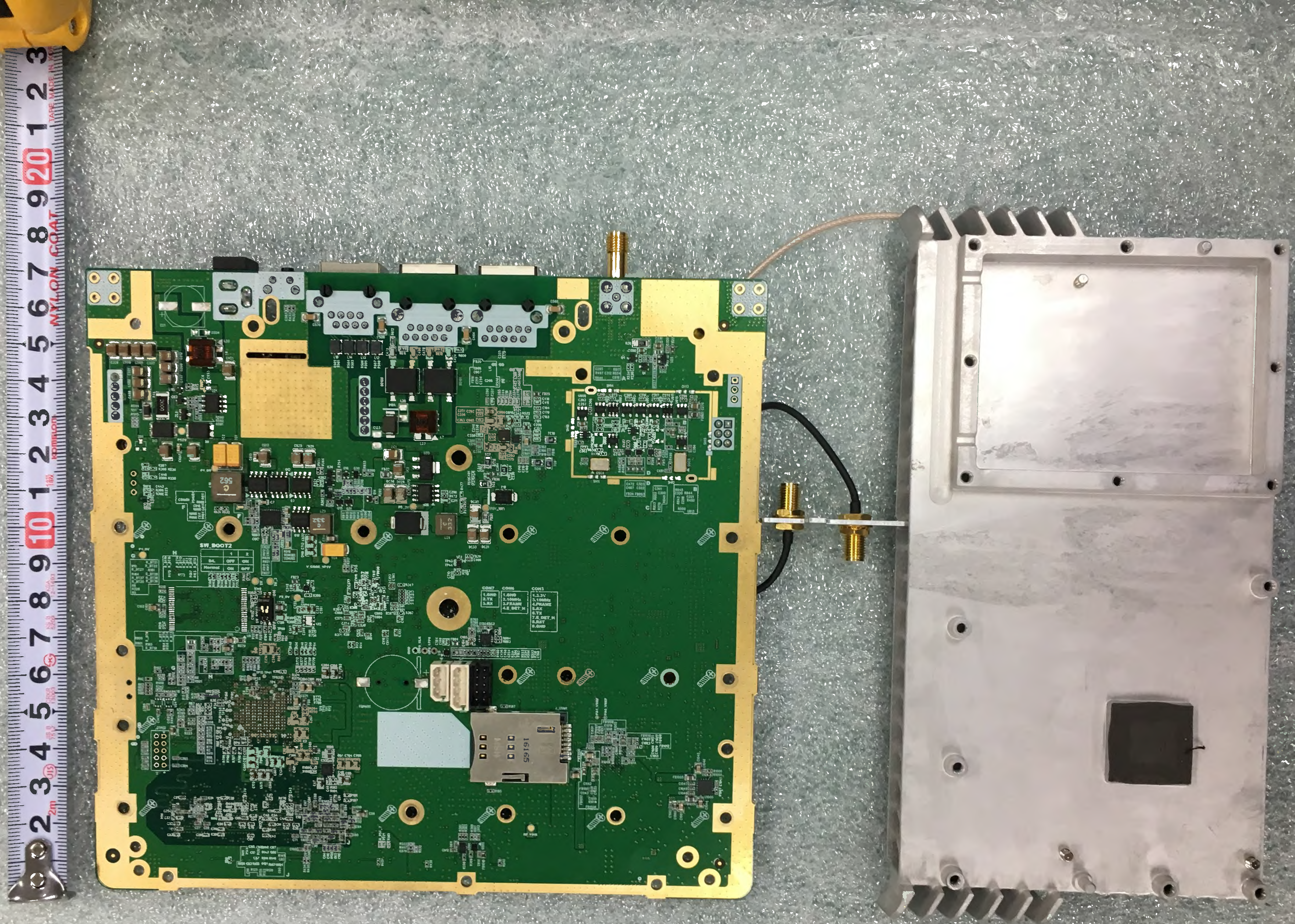
Back of PCB
