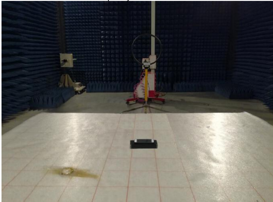
Radiated Spurious Emissions Test Frequency From 9KHz-30MHz
