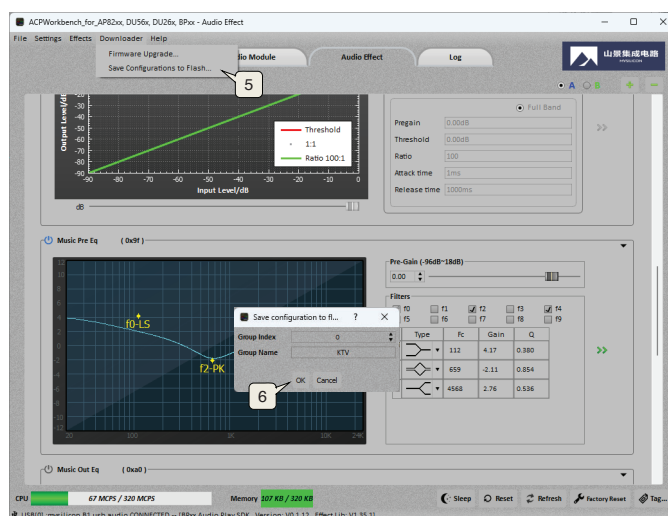
Figure 5: Save operation.
