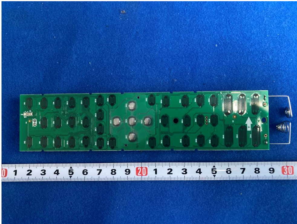
FIGURE 17 REMOTE CONTROL (ERF3ZB80) MAINBOARD BACK
