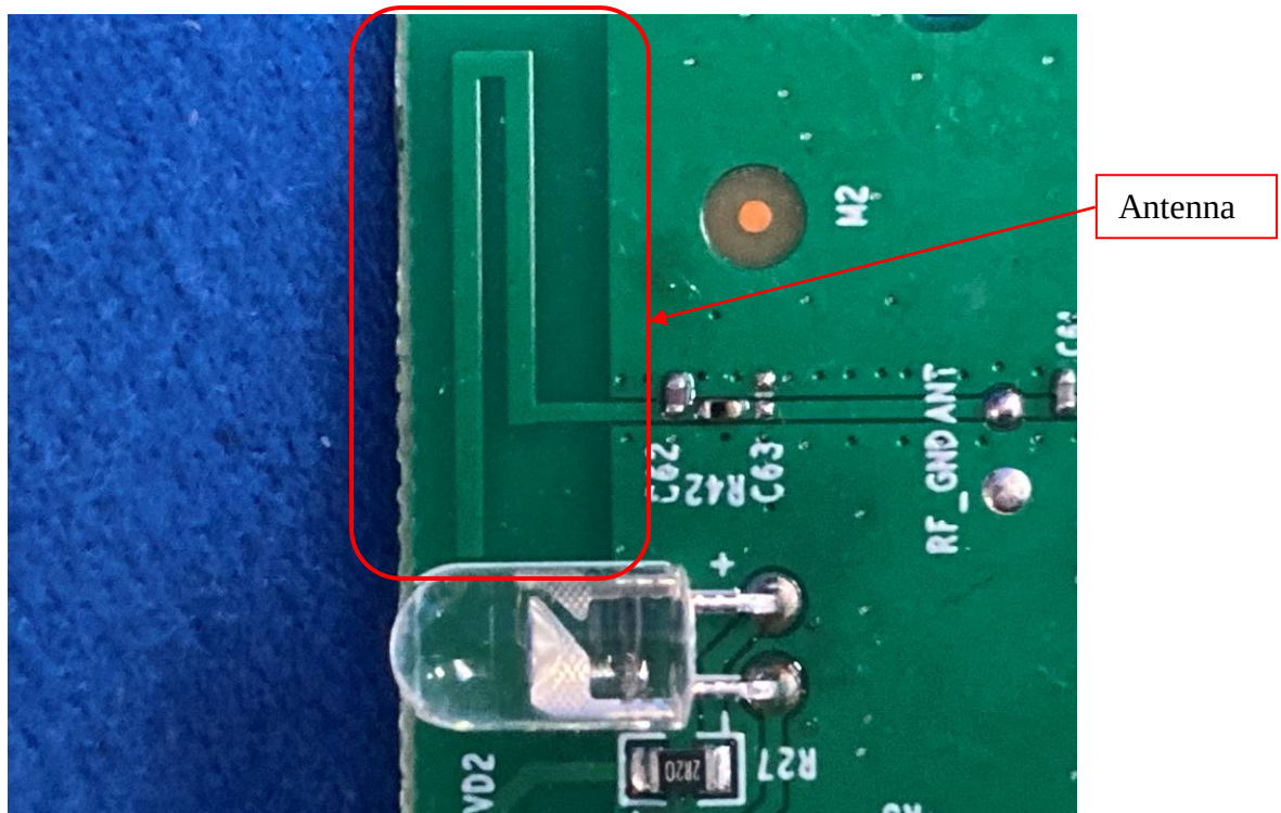
FIGURE 19 REMOTE CONTROL (ERF3ZB80) ANTENNA
