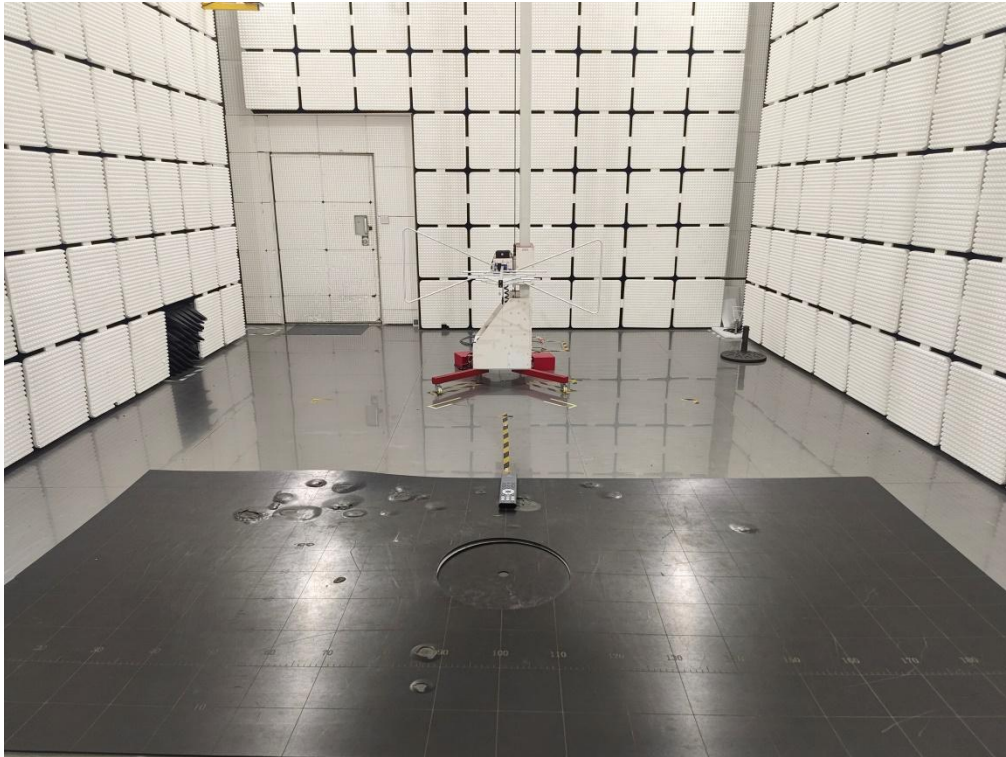
Emissions in Restricted Frequency Bands
