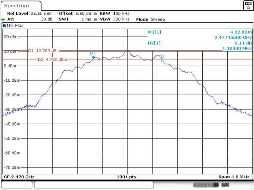
6 dB Bandwidth Plot on Channel 38
