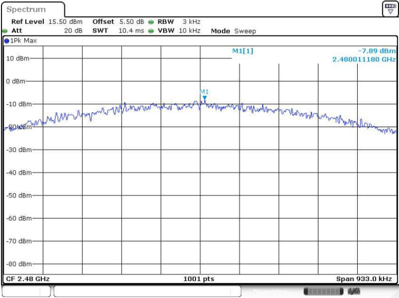
PSD 3kHz Plot on Channel 39
