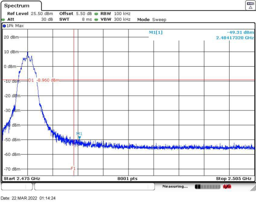
High Band Edge Plot on Channel 38
