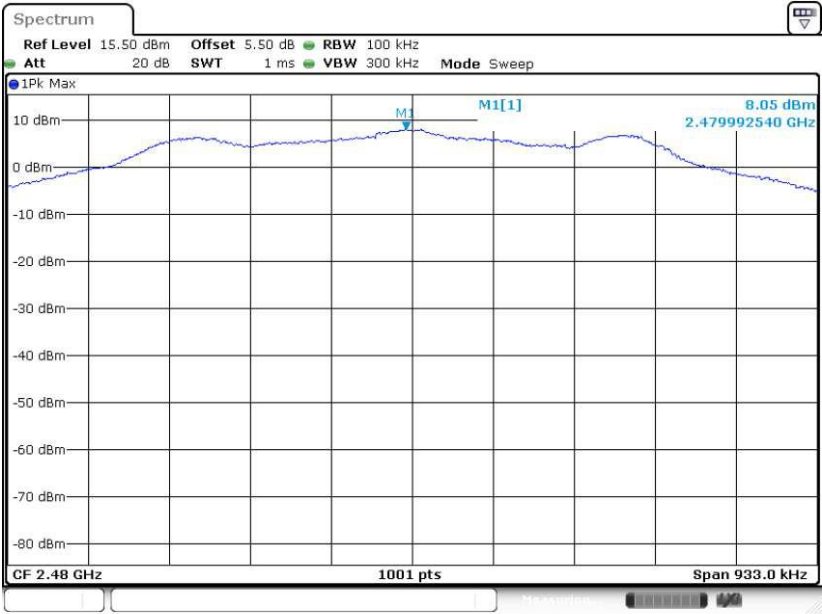
PSD 100kHz Plot on Channel 39
