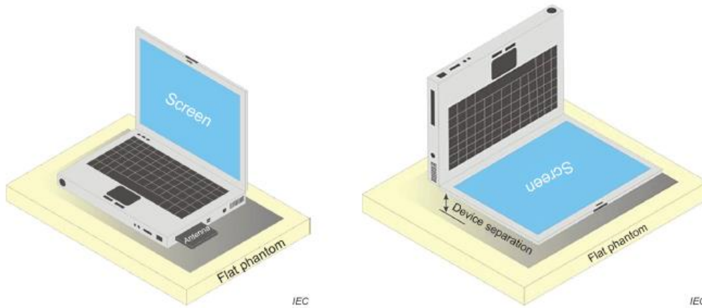
Fig.11.5 Illustration for Body Worn Position
