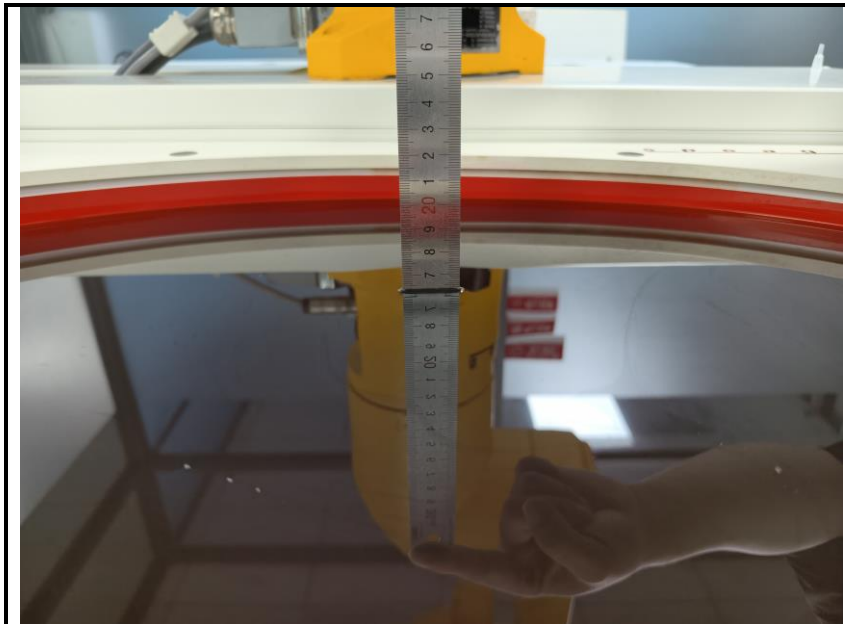
Fig. 9.4 Photo of Liquid Height for Body SAR (depth>15cm)
