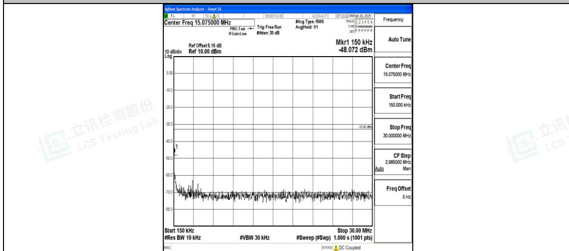
Band4_1.4MHz_16QAM_20393_1RB#0_0.15~30_0.15~30
