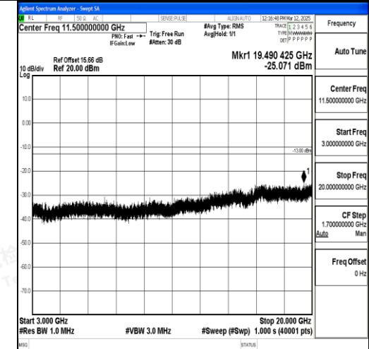
Band2_10MHz_16QAM_18650_1RB#0_3000~20 000_3000~20000
