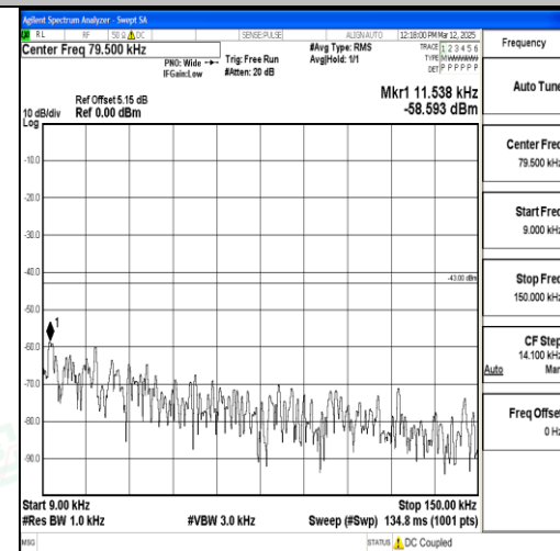
Band2_10MHz_QPSK_19150_1RB#0_0.009~0.15_0.009~0.15
