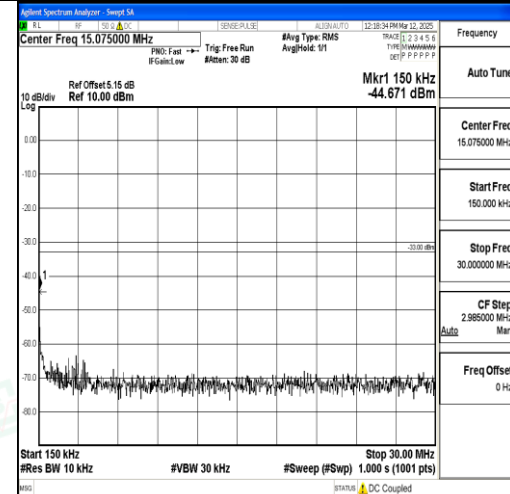
Band2_10MHz_16QAM_19150_1RB#0_0.15~3 0_0.15~30
