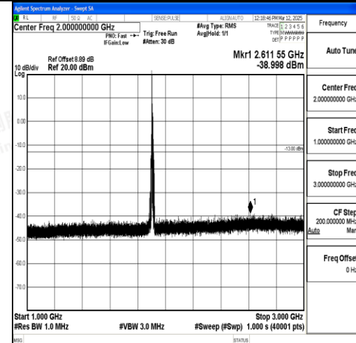
Band2_10MHz_16QAM_19150_1RB#0_1000~3 000_1000~3000
