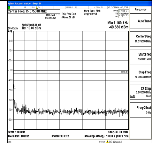
Band2_10MHz_QPSK_18900_1RB#0_0.15~30 0.15~30
