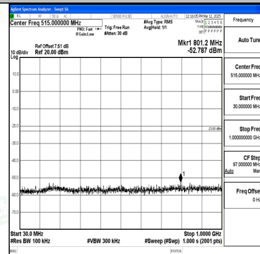
Band2_10MHz_QPSK_18650_1RB#0_30~1000 _30~1000
