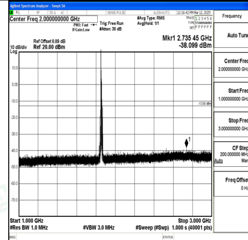
Band2_10MHz_16QAM_18650_1RB#0_1000~3 000_1000~3000
