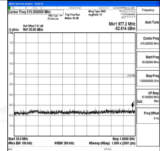
Band2_10MHz_16QAM_19150_1RB#0_30~1000 _30~1000
