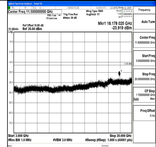
Band2_10MHz_16QAM_19150_1RB#0_3000~20 000_3000~20000
