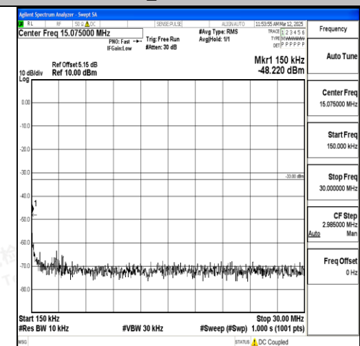
Band2_5MHz_QPSK_18625_1RB#0_0.15~30_0.15~30
