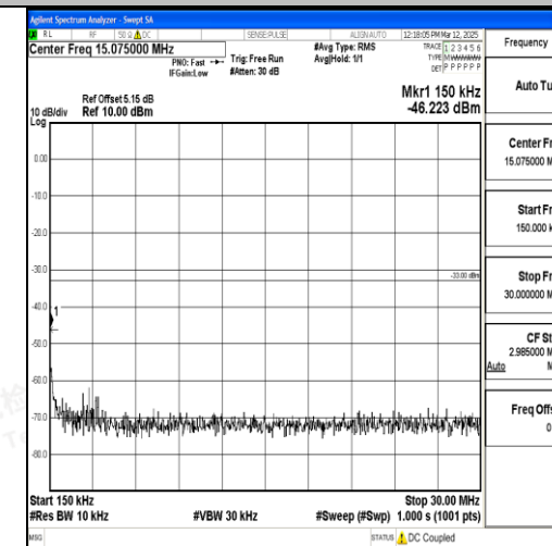
Band2_10MHz_QPSK_19150_1RB#0_0.15~30_0.15~30
