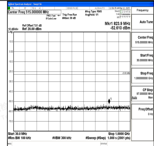
Band2_5MHz_16QAM_19175_1RB#0_30~1000 30~1000
