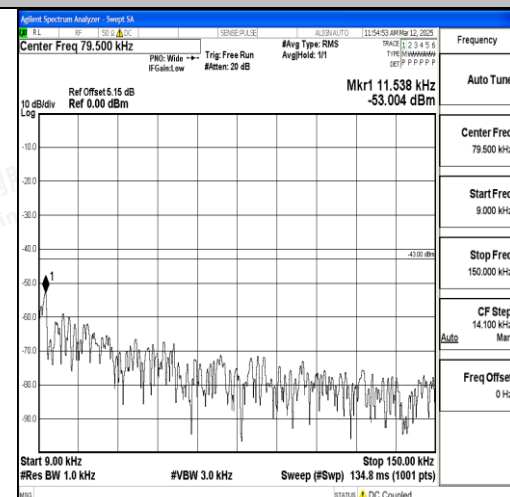
Band2_5MHz_QPSK_18900_1RB#0_0.009~0.15_0.009~0.15
