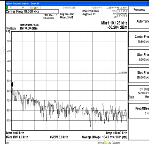
Band2_10MHz_QPSK_18900_1RB#0_0.009~0. 15_0.009~0.15
