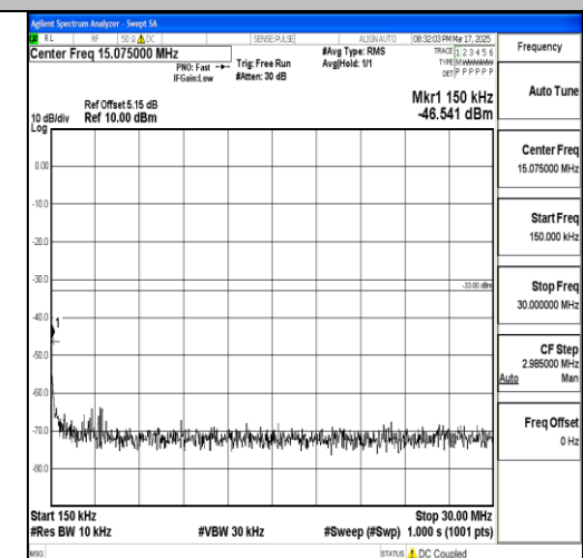
Band2_3MHz_16QAM_19185_1RB#0_0.15~30_0.15~30
