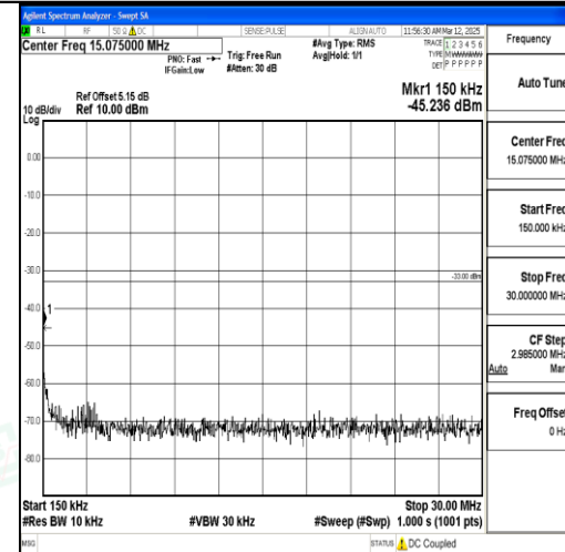
Band2_5MHz_16QAM_19175_1RB#0_0.15~30 _0.15~30
