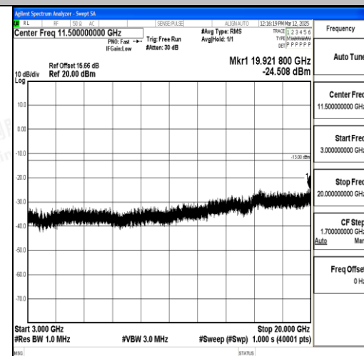
Band2_10MHz_QPSK_18650_1RB#0_3000~20 000_3000~20000
