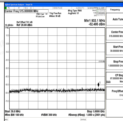
Band2_10MHz_QPSK_19150_1RB#0_30~1000_30~1000
