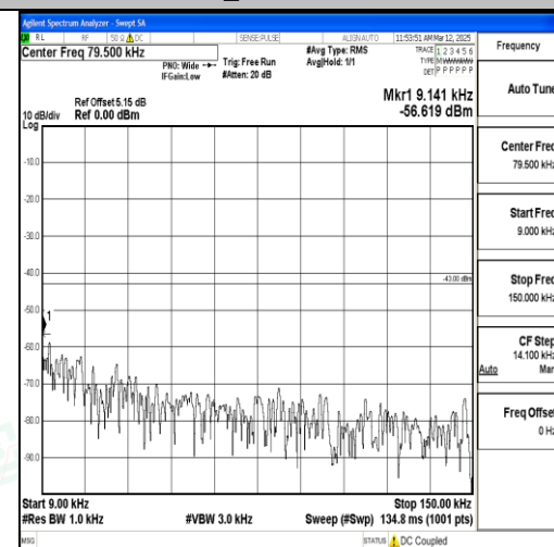
Band2_5MHz_QPSK_18625_1RB#0_0.009~0.15
