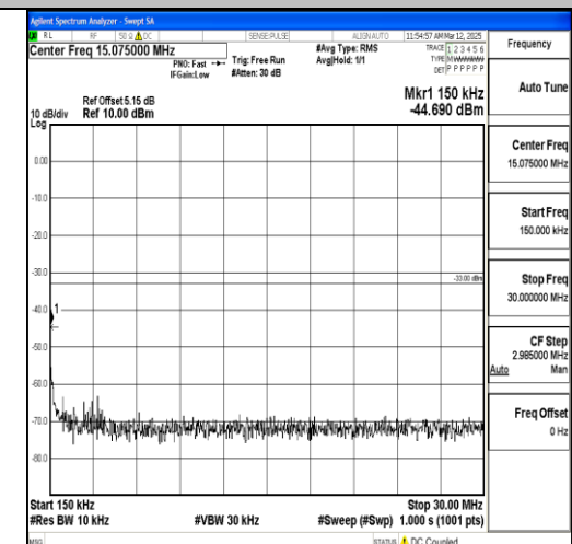
Band2_5MHz_QPSK_18900_1RB#0_0.15~30_0.15~30
