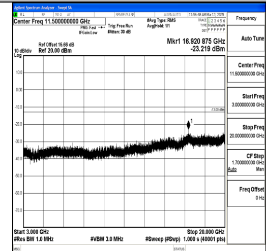
Band2_5MHz_16QAM_19175_1RB#0_3000~200 00_3000~20000
