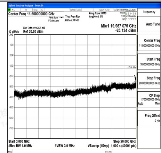
Band2_5MHz_16QAM_18625_1RB#0_3000~20000_3000~20000
