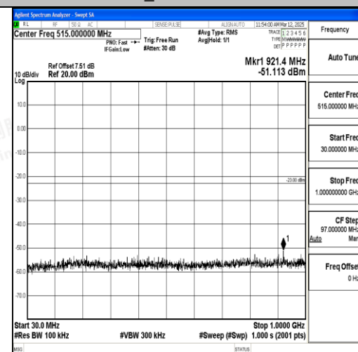
Band2_5MHz_QPSK_18625_1RB#0_30~1000_30~1000
