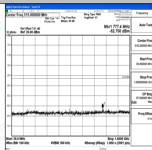
Band2_5MHz_QPSK_18625_1RB#0_30~1000_30~1000
