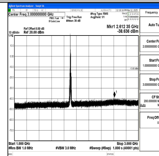
Band2_10MHz_QPSK_19150_1RB#0_1000~3000_0_1000~3000
