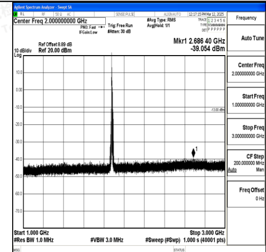
Band2_10MHz_QPSK_18900_1RB#0_0.15~30 0.15~30
