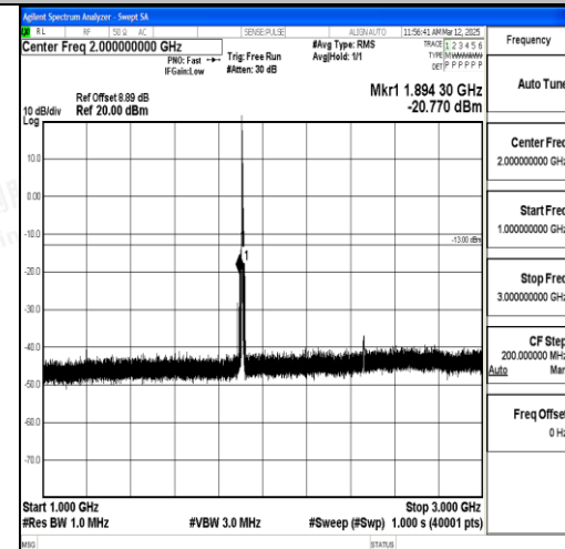
Band2_5MHz_16QAM_19175_1RB#0_1000~30 00_1000~3000
