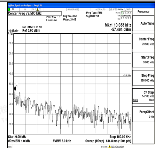
Band2_15MHz_16QAM_18900_1RB#0_0.009~0. 15_0.009~0.15
