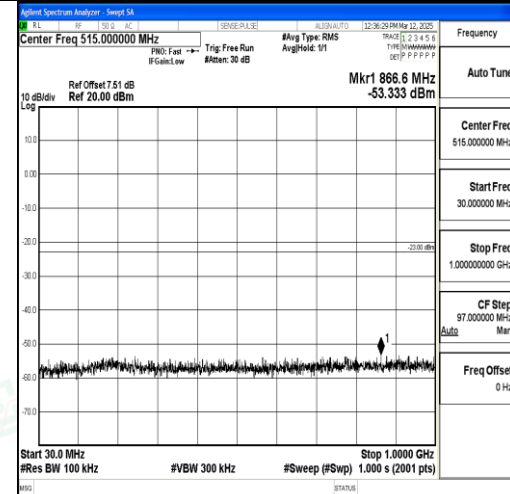
Band2_15MHz_QPSK_18675_1RB#0_30~1000 _30~1000
