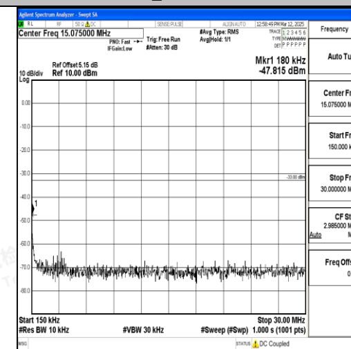
Band2_20MHz_QPSK_19100_1RB#0_0.15~30_0.15~30
