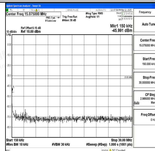
Band2_15MHz_16QAM_18900_1RB#0_0.15~3 0_0.15~30
