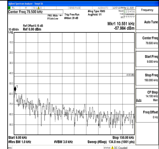
Band2_20MHz_16QAM_18700_1RB#0_0.009~0. 15_0.009~0.15
