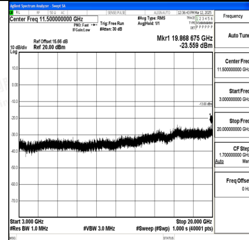
Band2_15MHz_QPSK_18675_1RB#0_3000~20 000_3000~20000
