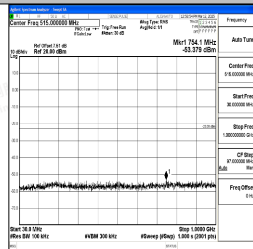
Band2_20MHz_QPSK_19100_1RB#0_30~1000_30~1000
