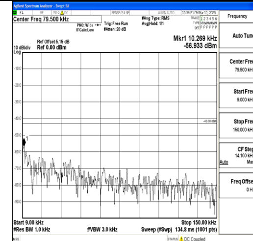
Band2_15MHz_16QAM_18675_1RB#0_0.009~0. 15_0.009~0.15
