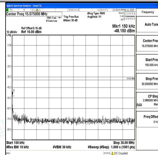
Band2_15MHz_16QAM_19125_1RB#0_0.15~3 0_0.15~30
