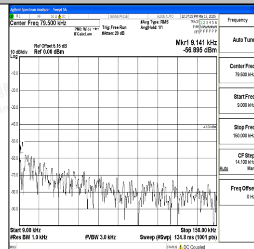
Band2_15MHz_QPSK_18900_1RB#0_0.009~0. 15_0.009~0.15
