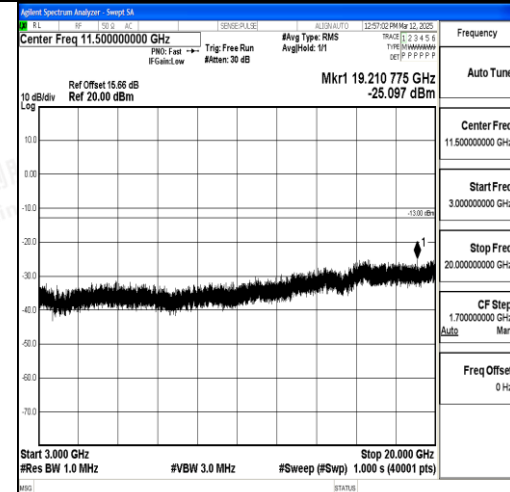
Band2_20MHz_QPSK_18700_1RB#0_3000~20 000_3000~20000
