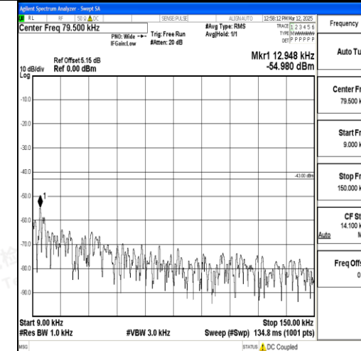
Band2_20MHz_16QAM_18900_1RB#0_0.009~0. 15_0.009~0.15
