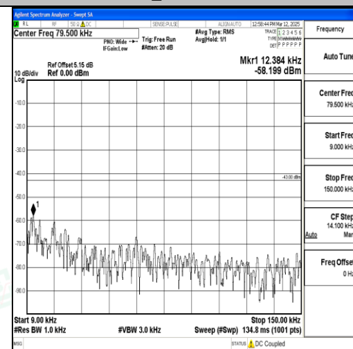
Band2_20MHz_QPSK_19100_1RB#0_0.009~0.15_0.009~0.15
