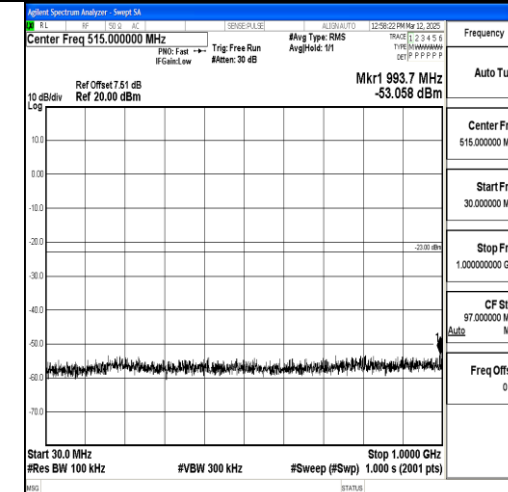
Band2_20MHz_16QAM_18900_1RB#0_30~1000 _30~1000
