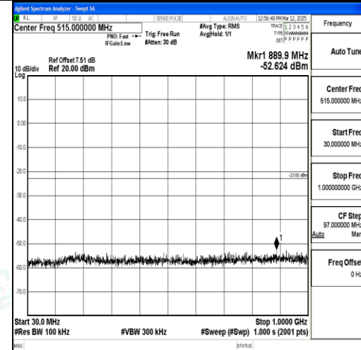
Band2_20MHz_QPSK_18700_1RB#0_30~1000 _30~1000
