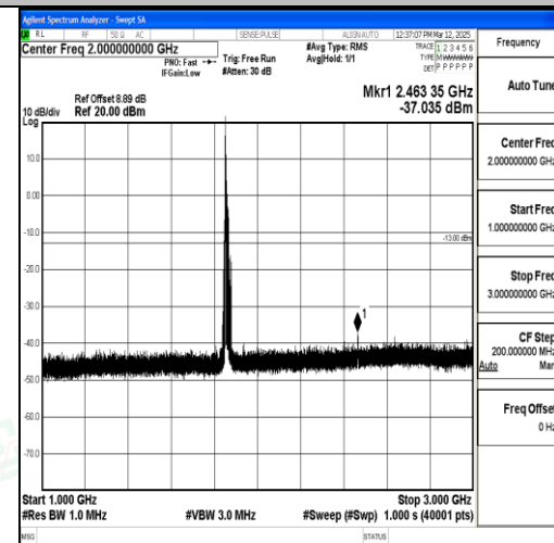
Band2_15MHz_16QAM_18675_1RB#0_1000~3 000_1000~3000
