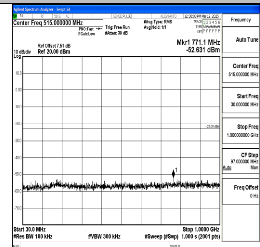
Band2_15MHz_16QAM_18900_1RB#0_30~1000 _30~1000
