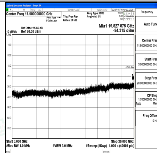
Band2_15MHz_QPSK_18900_1RB#0_3000~20 000_3000~20000
