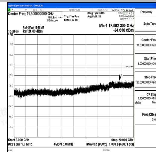
Band2_15MHz_16QAM_18675_1RB#0_3000~20 000_3000~20000
