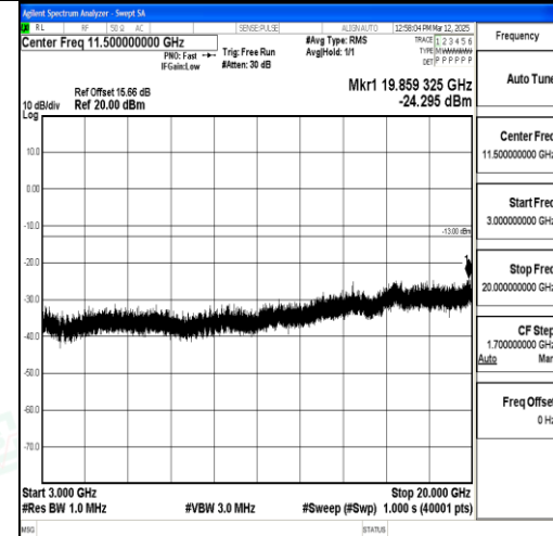
Band2_20MHz_QPSK_18900_1RB#0_3000~20 000_3000~20000
