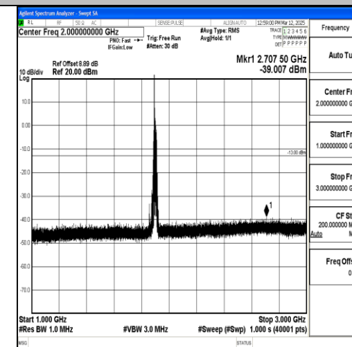
Band2_20MHz_QPSK_19100_1RB#0_1000~3000_0_1000~3000
