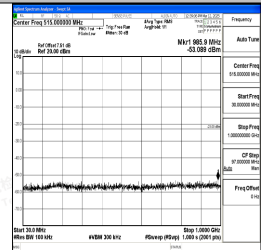
Band2_15MHz_16QAM_19125_1RB#0_30~1000 _30~1000
