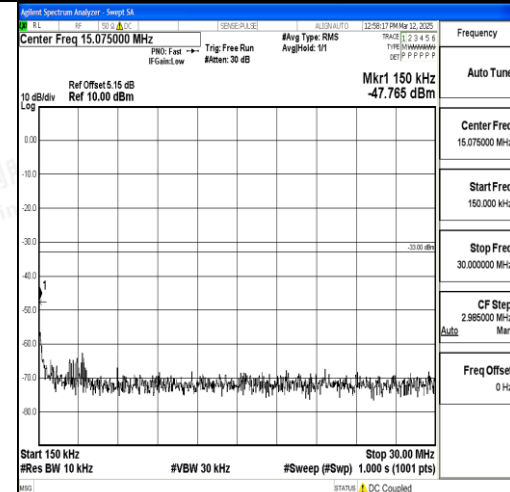
Band2_20MHz_16QAM_18900_1RB#0_0.15~3 0_0.15~30
