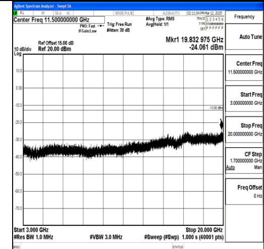
Band4_5MHz_16QAM_20375_1RB#0_3000~200 00_3000~20000
