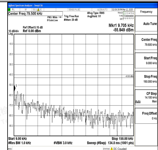
Band4_5MHz_16QAM_20175_1RB#0_0.009~0.15_0.009~0.15
