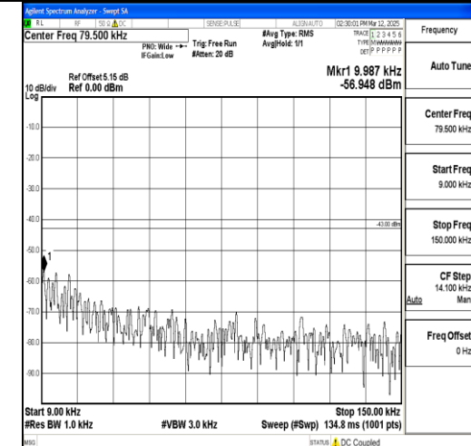
Band4_10MHz_16QAM_20000_1RB#0_0.009~0.15_15_0.009~0.15
