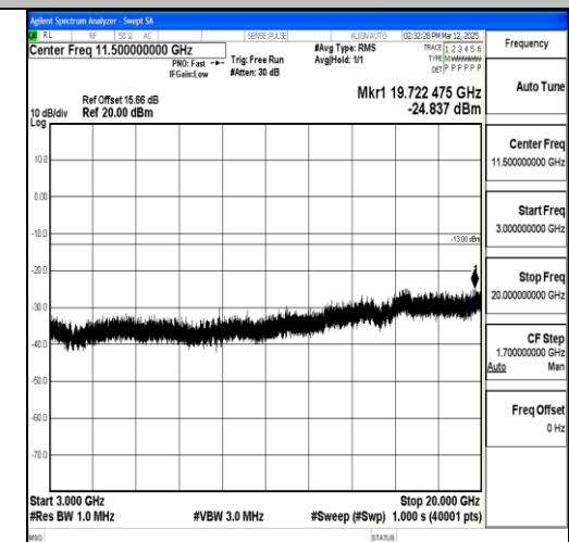
Band4_10MHz_16QAM_20350_1RB#0_3000~20 000_3000~20000
