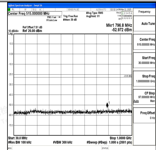
Band4_10MHz_16QAM_20350_1RB#0_30~1000 _30~1000
