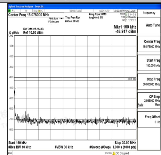
Band4_3MHz_QPSK_20385_1RB#0_0.15~30_0. 15~30
