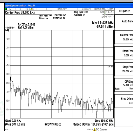
Band4_3MHz_QPSK_20385_1RB#0_0.009~0.1 5_0.009~0.15
