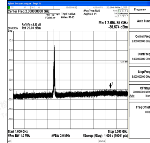
Band4_10MHz_QPSK_20000_1RB#0_1000~3000_0_1000~3000
