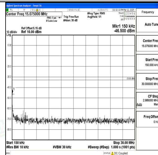
Band4_10MHz_16QAM_20350_1RB#0_0.15~3 0_0.15~30
