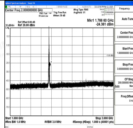
Band4_5MHz_16QAM_20375_1RB#0_1000~30 00_1000~3000
