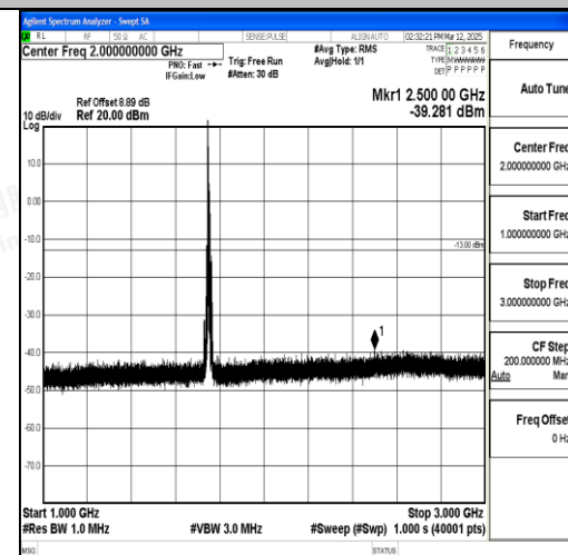
Band4_10MHz_16QAM_20350_1RB#0_1000~3 000_1000~3000
