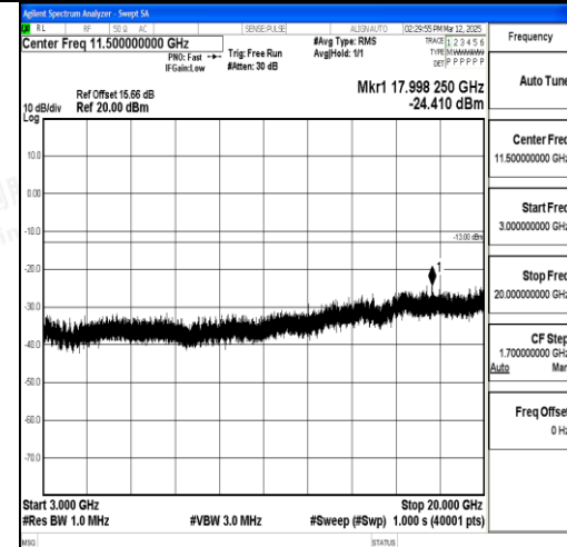
Band4_10MHz_QPSK_20000_1RB#0_3000~20000_000_3000~20000
