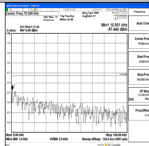
Band4_15MHz_QPSK_20175_1RB#0_0.009~0. 15_0.009~0.15
