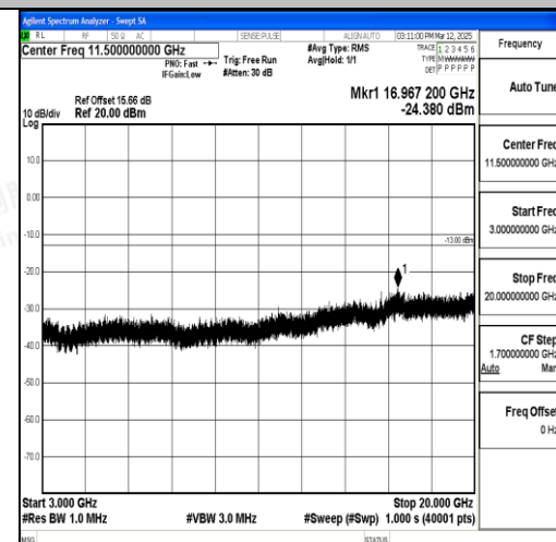
Band4_20MHz_QPSK_20050_1RB#0_3000~20 000_3000~20000
