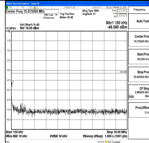
Band4_20MHz_16QAM_20175_1RB#0_0.15~3 0_0.15~30
