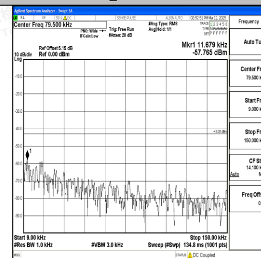
Band4_15MHz_QPSK_20325_1RB#0_1000~3000_0_1000~3000
