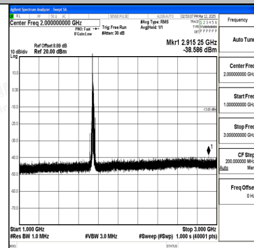
Band4_15MHz_16QAM_20325_1RB#0_1000~3 000_1000~3000
