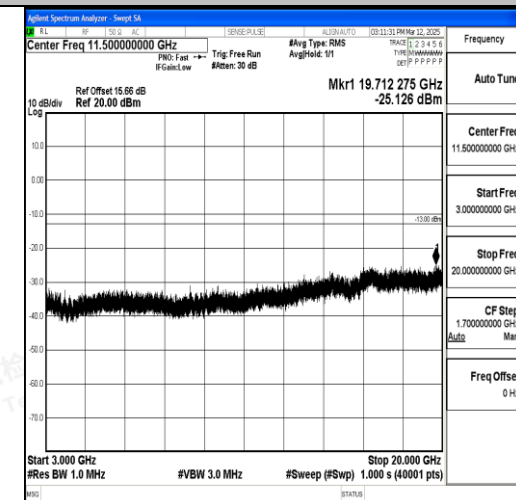
Band4_20MHz_16QAM_20050_1RB#0_3000~20 000_3000~20000
