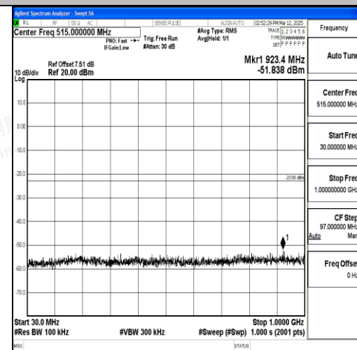
Band4_15MHz_QPSK_20325_1RB#0_30~1000_30~1000
