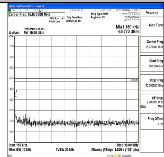
Band4_15MHz_QPSK_20175_1RB#0_0.15~30 0.15~30
