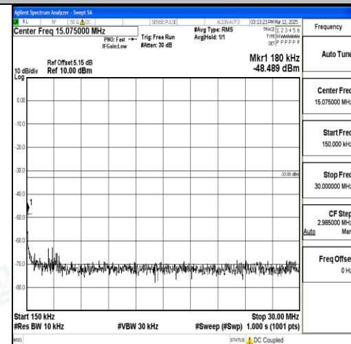
Band4_20MHz_16QAM_20300_1RB#0_0.15~30_0.15~30
