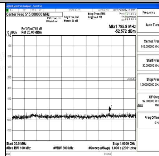
Band4_20MHz_QPSK_20300_1RB#0_30~1000_30~1000
