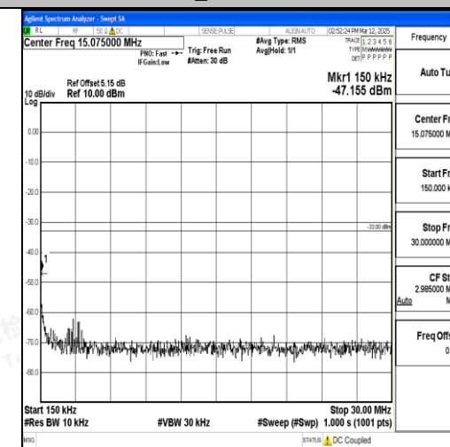
Band4_15MHz_QPSK_20325_1RB#0_0.15~30_0.15~30
