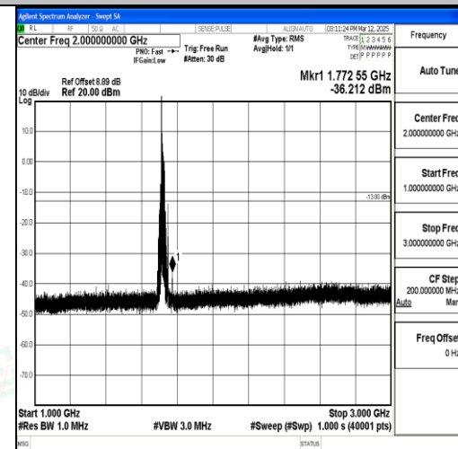
Band4_20MHz_16QAM_20050_1RB#0_1000~3 000_1000~3000
