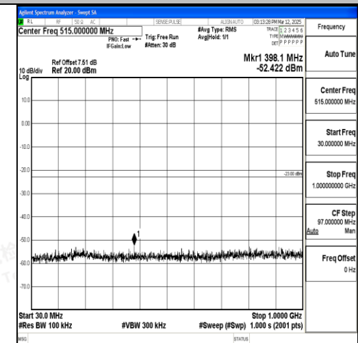
Band4_20MHz_16QAM_20300_1RB#0_30~1000_30~1000
