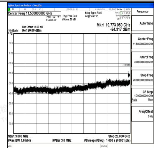
Band4_15MHz_16QAM_20025_1RB#0_3000~20 000_3000~20000
