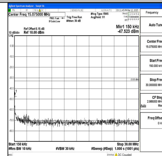
Band4_20MHz_QPSK_20175_1RB#0_0.15~30 0.15~30
