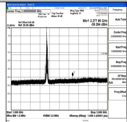
Band4_20MHz_QPSK_20300_1RB#0_1000~3000_0_1000~3000
