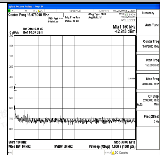
Band4_20MHz_QPSK_20300_1RB#0_0.15~30_0.15~30
