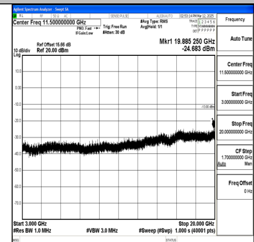
Band4_15MHz_16QAM_20325_1RB#0_3000~20 000_3000~20000
