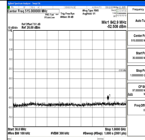
Band4_20MHz_16QAM_20175_1RB#0_30~1000 _30~1000
