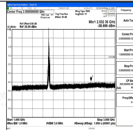
Band4_15MHz_QPSK_20025_1RB#0_1000~300 0_1000~3000
