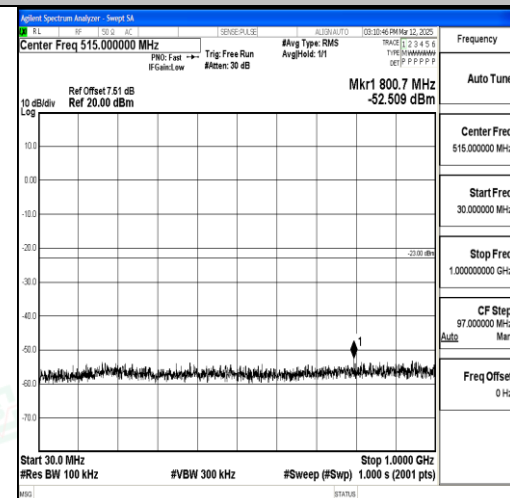
Band4_20MHz_QPSK_20050_1RB#0_30~1000 _30~1000
