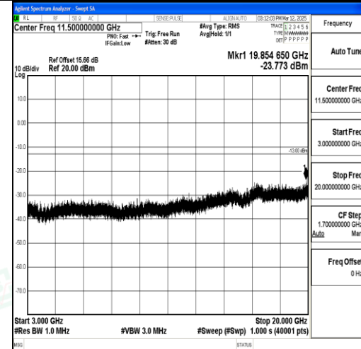
Band4_20MHz_QPSK_20175_1RB#0_3000~20 000_3000~20000
