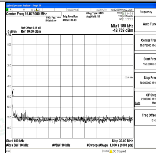
Band4_15MHz_16QAM_20325_1RB#0_0.15~3 0_0.15~30
