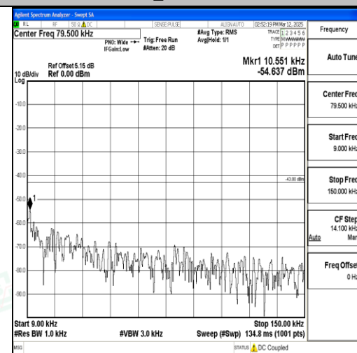
Band4_15MHz_QPSK_20325_1RB#0_0.009~0.15_0.009~0.15
