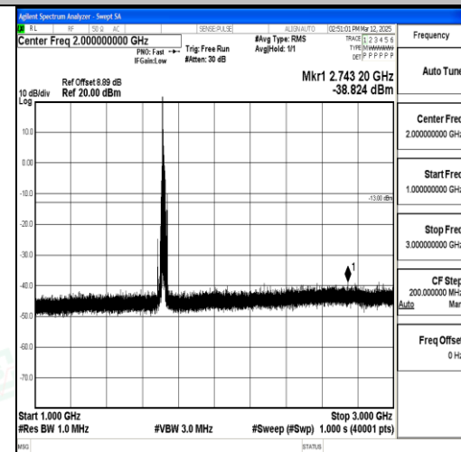
Band4_15MHz_16QAM_20025_1RB#0_1000~3 000_1000~3000
