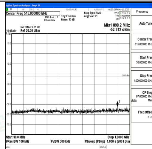
Band4_15MHz_QPSK_20025_1RB#0_30~1000 _30~1000
