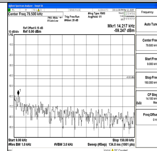
Band4_20MHz_16QAM_20050_1RB#0_0.009~0. 15_0.009~0.15
