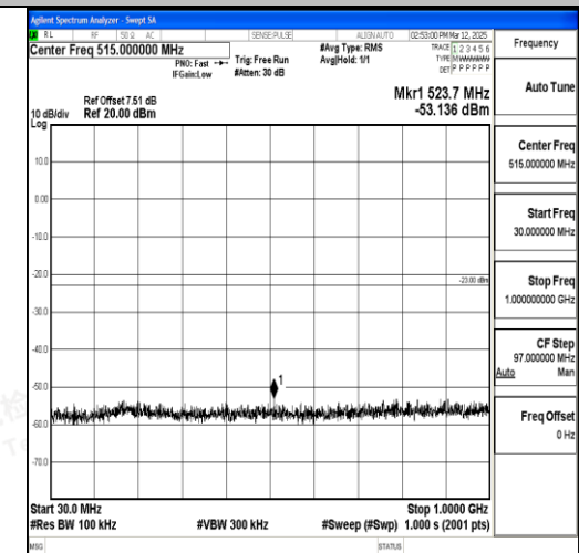
Band4_15MHz_16QAM_20325_1RB#0_30~1000 _30~1000
