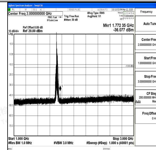
Band4_20MHz_QPSK_20050_1RB#0_1000~300 0_1000~3000
