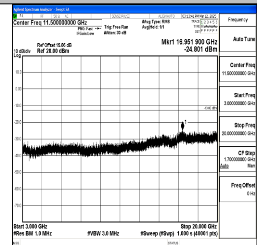
Band4_20MHz_16QAM_20300_1RB#0_3000~20000_3000~20000
