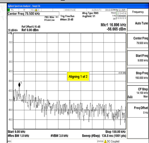
Band4_20MHz_QPSK_20300_1RB#0_1000~3000_0_1000~3000
