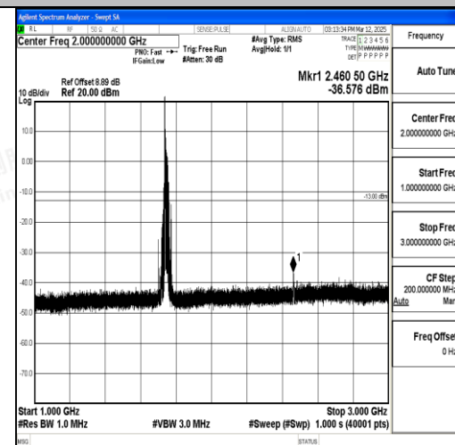
Band4_20MHz_16QAM_20300_1RB#0_1000~3000_1000~3000
