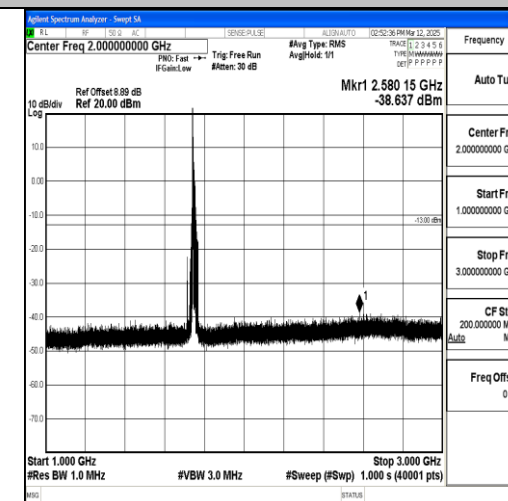
Band4_15MHz_QPSK_20325_1RB#0_1000~3000_0_1000~3000
