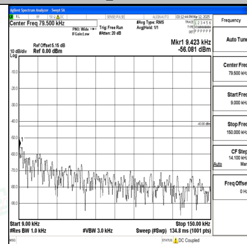
Band4_20MHz_QPSK_20300_1RB#0_0.009~0.15_0.009~0.15
