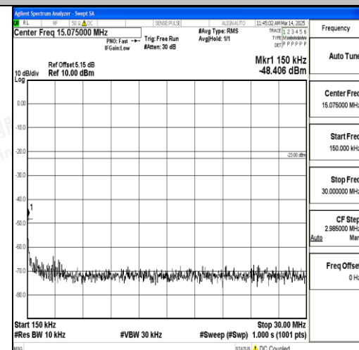
Band17_5MHz_16QAM_23790_1RB#0_0.15~3 0_0.15~30
