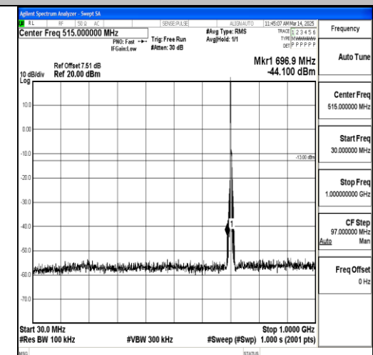
Band17_5MHz_16QAM_23790_1RB#0_30~1000 _30~1000
