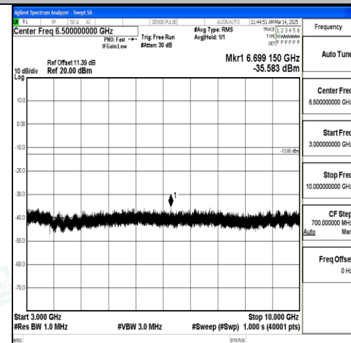
Band17_5MHz_QPSK_23790_1RB#0_3000~10 000_3000~10000
