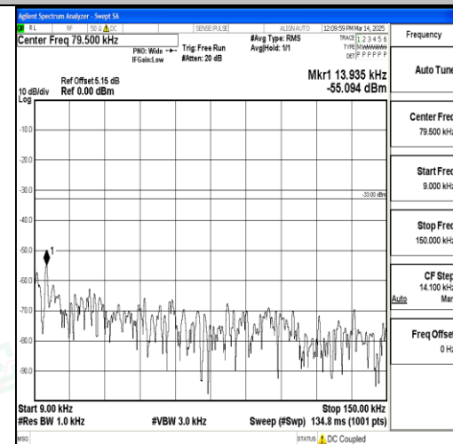
Band17_10MHz_QPSK_23800_1RB#0_0.009~0.15_0.009~0.15
