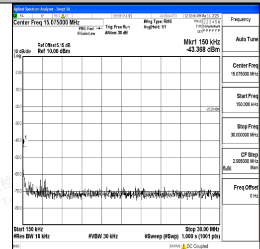
Band17_10MHz_QPSK_23800_1RB#0_0.15~30_0.15~30
