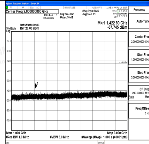
Band17_5MHz_16QAM_23825_1RB#0_1000~3 000_1000~3000
