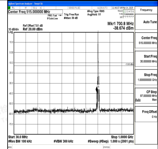
Band17_5MHz_16QAM_23825_1RB#0_30~1000 _30~1000
