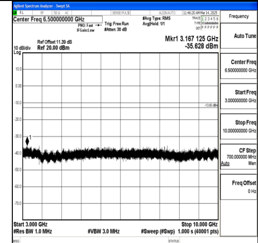
Band17_5MHz_16QAM_23825_1RB#0_3000~10 000_3000~10000
