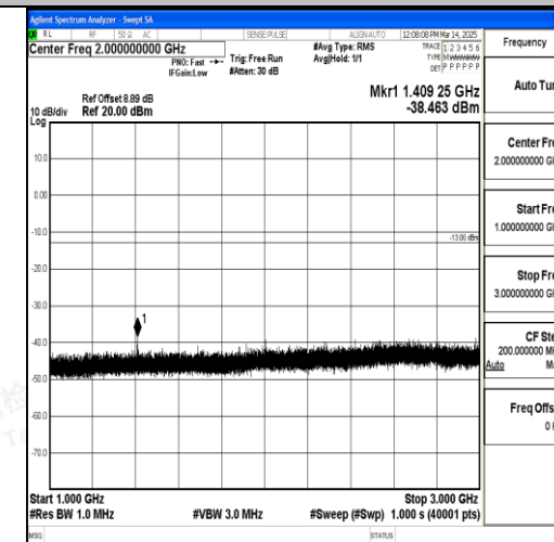
Band17_10MHz_QPSK_23780_1RB#0_1000~30 00_1000~3000
