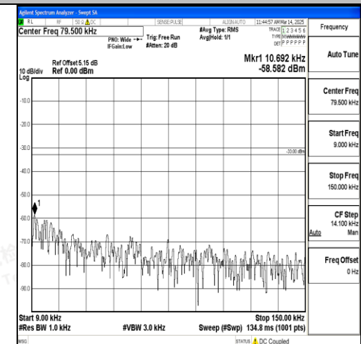
Band17_5MHz_16QAM_23790_1RB#0_0.009~0. 15_0.009~0.15
