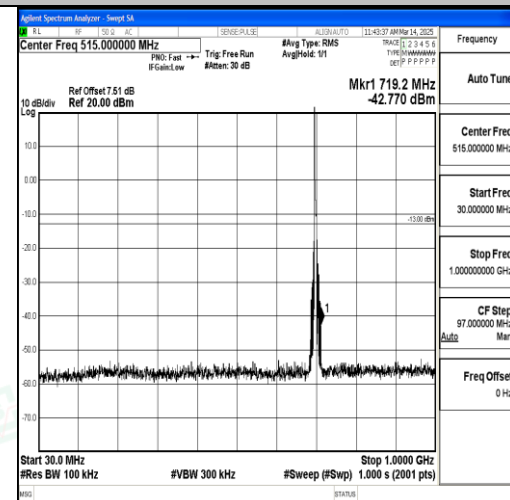
Band17_5MHz_QPSK_23755_1RB#0_30~1000 _30~1000
