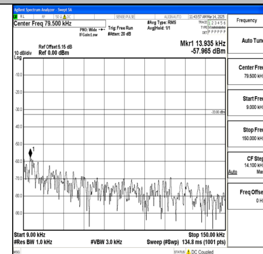
Band17_5MHz_16QAM_23755_1RB#0_0.009~0. 15_0.009~0.15
