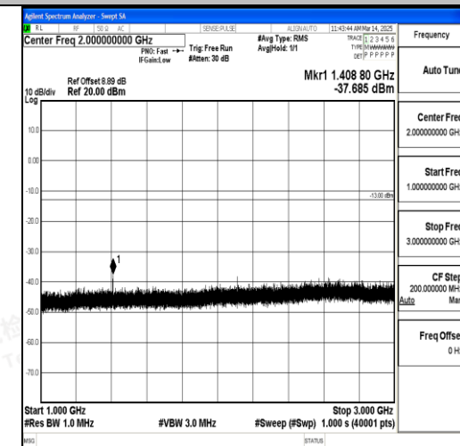
Band17_5MHz_QPSK_23755_1RB#0_1000~300 0_1000~3000
