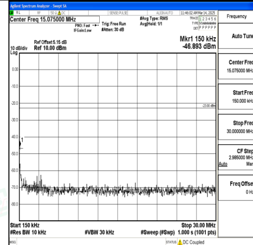
Band17_5MHz_16QAM_23825_1RB#0_0.15~3 0_0.15~30
