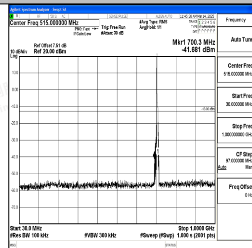
Band17_5MHz_QPSK_23825_1RB#0_30~1000_30~1000
