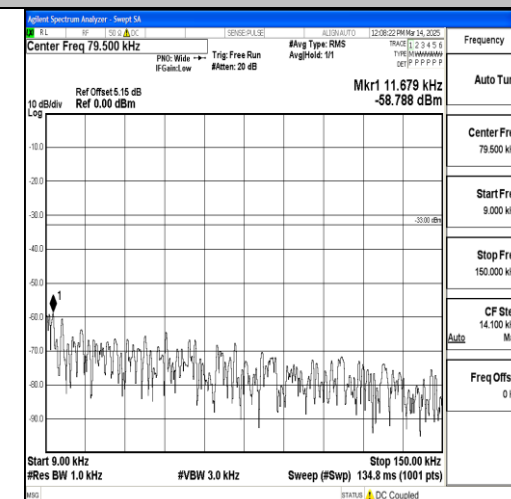
Band17_10MHz_16QAM_23780_1RB#0_0.009~ 0.15_0.009~0.15
