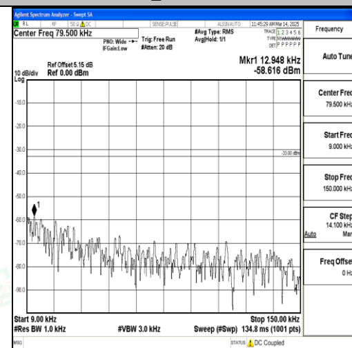
Band17_5MHz_QPSK_23825_1RB#0_0.009~0.15_0.009~0.15
