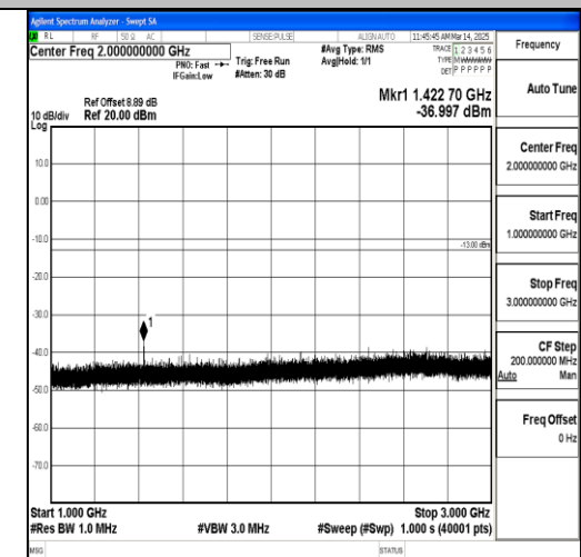
Band17_5MHz_QPSK_23825_1RB#0_1000~3000_0_1000~3000
