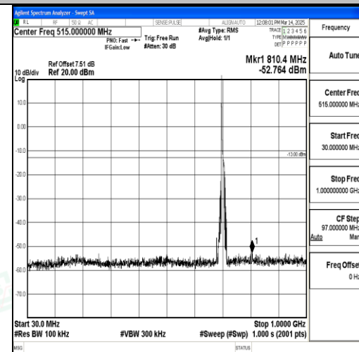
Band17_10MHz_QPSK_23780_1RB#0_30~100 0_30~1000
