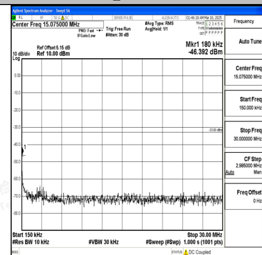
Band66_3MHz_16QAM_132322_1RB#0_0.15~30_0_0.15~30
