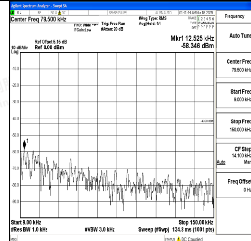
Band66_1.4MHz_QPSK_132322_1RB#0_0.009 ~0.15_0.009~0.15
