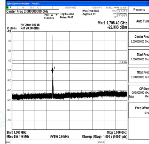
Band66_1.4MHz_16QAM_131979_1RB#0_1000 ~3000_1000~3000
