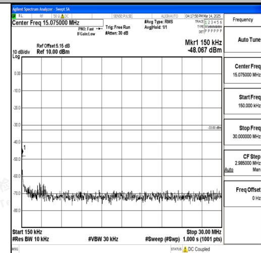
Band66_10MHz_16QAM_132322_1RB#0_0.15~ 30_0.15~30
