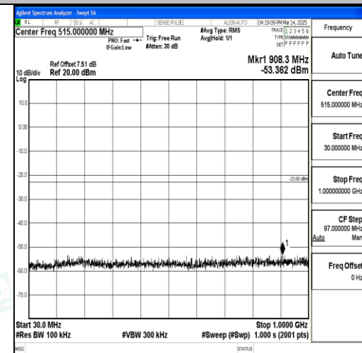
Band66_10MHz_16QAM_132622_1RB#0_30~1 000_30~1000
