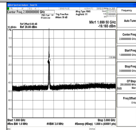
Band66_5MHz_QPSK_131997_1RB#0_1000~3 000_1000~3000
