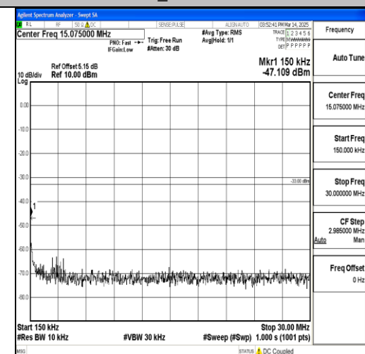
Band66_5MHz_16QAM_131997_1RB#0_0.15~3 0_0.15~30
