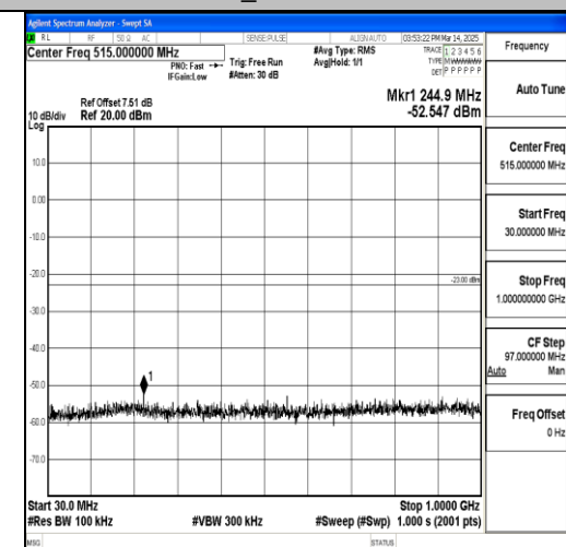
Band66_5MHz_QPSK_132322_1RB#0_30~1000 0_30~1000
