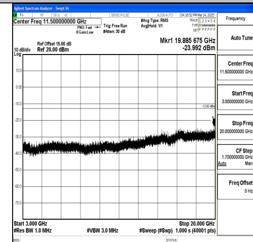
Band66_10MHz_QPSK_132622_1RB#0_3000~ 20000_3000~20000
