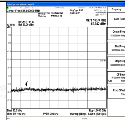
Band66_10MHz_QPSK_132622_1RB#0_30~10 00_30~1000
