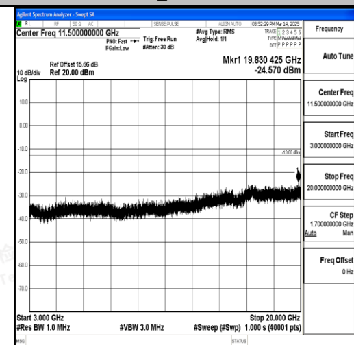
Band66_5MHz_QPSK_131997_1RB#0_3000~2 0000_3000~20000
