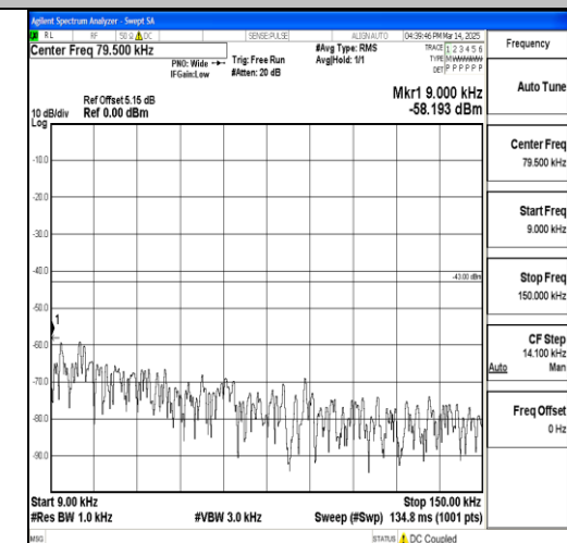
Band66_15MHz_QPSK_132047_1RB#0_0.009~ 0.15_0.009~0.15
