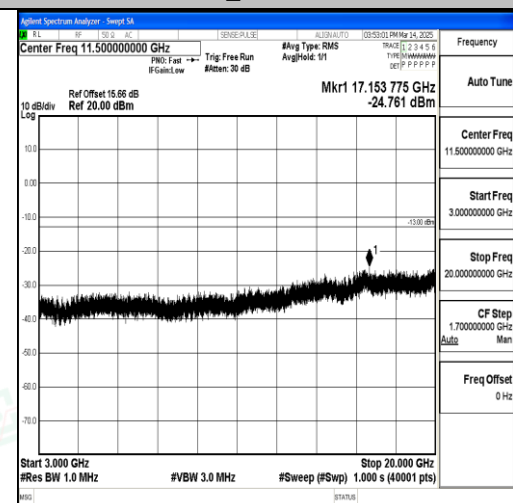
Band66_5MHz_16QAM_131997_1RB#0_3000~ 20000_3000~20000
