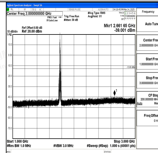
Band66_10MHz_QPSK_132622_1RB#0_1000~ 3000_1000~3000
