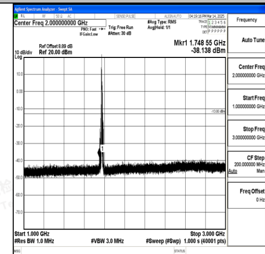
Band66_10MHz_16QAM_132622_1RB#0_1000 ~3000_1000~3000
