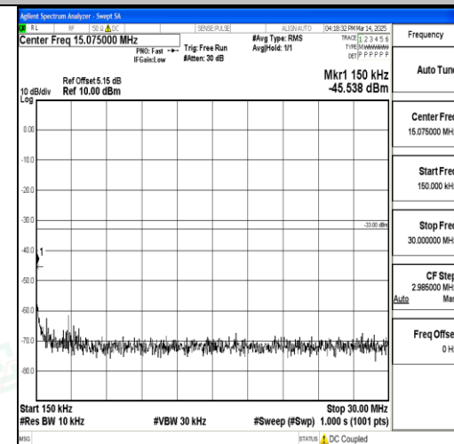
Band66_10MHz_QPSK_132622_1RB#0_0.15~3 0_0.15~30
