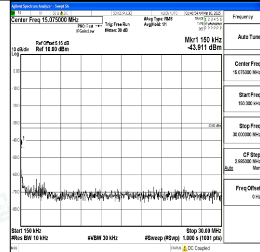
Band66_3MHz_QPSK_132657_1RB#0_0.15~30 _0.15~30
