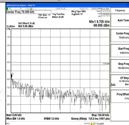
Band66_5MHz_QPSK_132322_1RB#0_0.009~0 .15_0.009~0.15
