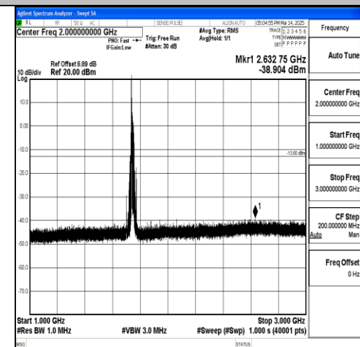
Band66_20MHz_16QAM_132322_1RB#0_1000~3000_1000~3000
