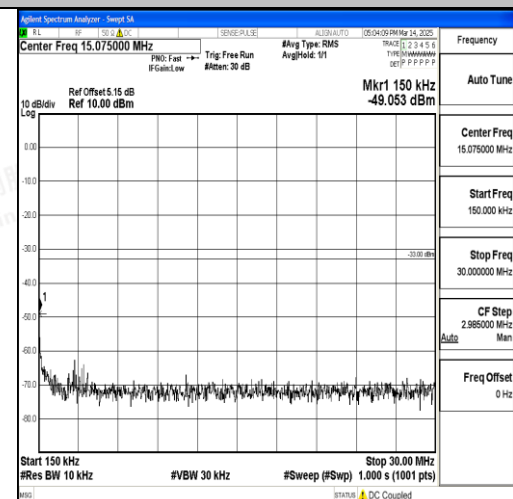
Band66_20MHz_QPSK_132322_1RB#0_0.15~3 0_0.15~30
