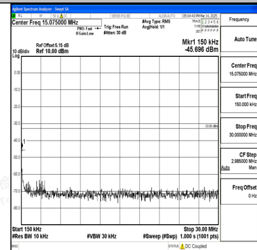
Band66_20MHz_16QAM_132322_1RB#0_0.15~30_0.15~30
