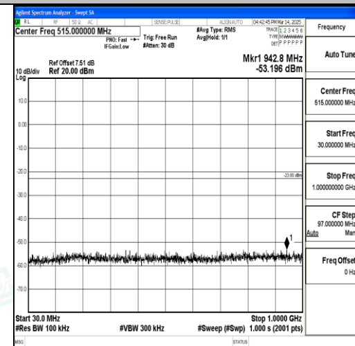
Band66_15MHz_16QAM_132597_1RB#0_30~1 000_30~1000
