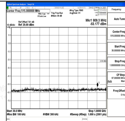
Band66_15MHz_QPSK_132597_1RB#0_30~10 00_30~1000
