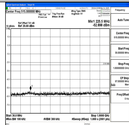
Band66_20MHz_QPSK_132322_1RB#0_30~10 00_30~1000
