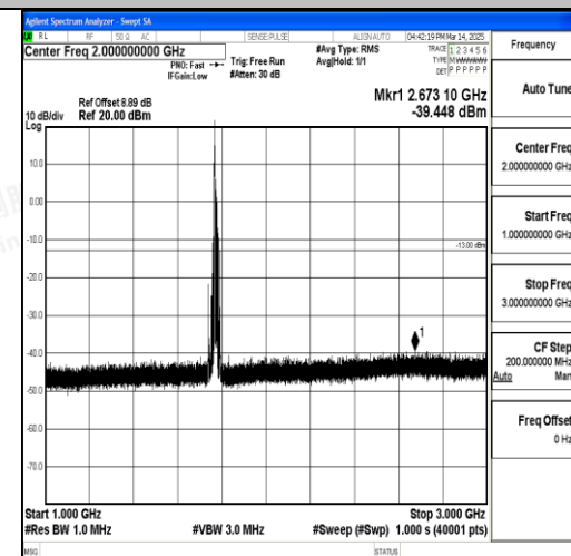
Band66_15MHz_QPSK_132597_1RB#0_1000~ 3000_1000~3000
