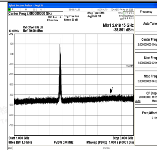
Band66_15MHz_16QAM_132597_1RB#0_1000 ~3000_1000~3000
