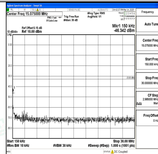
Band66_15MHz_QPSK_132597_1RB#0_0.15~3 0_0.15~30
