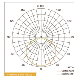
Photometric Data
