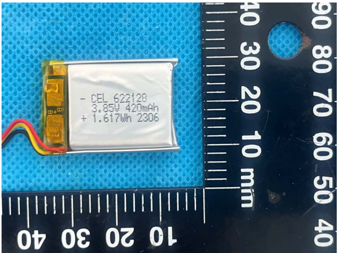
Charging Case Battery
