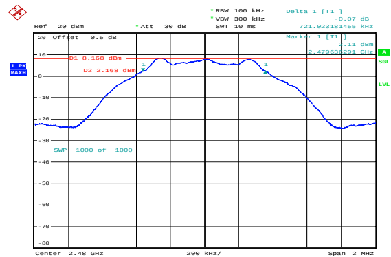
High 0.721MHz
