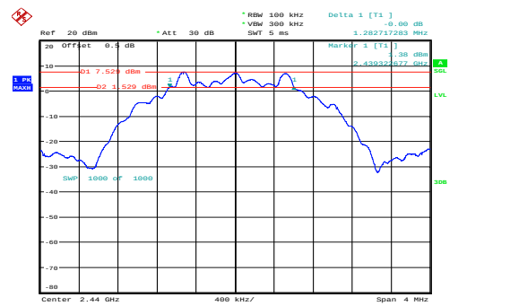
Middle 1.283MHz
