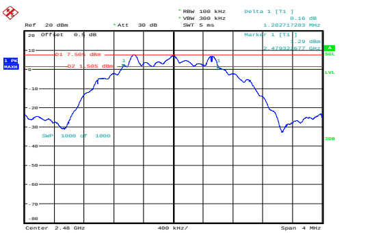
High 1.283MHz
