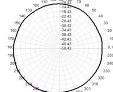
Total(H+V), Max=-10.73dB, CrD=5.12
