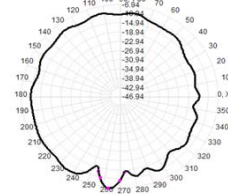
Total(H+V), Max=-10.44dB, CrD=6.21
