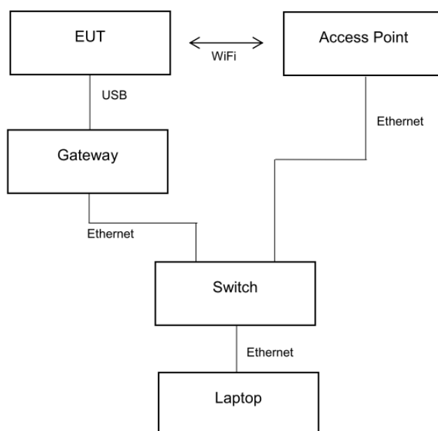
Figure 8 Block diagramm
