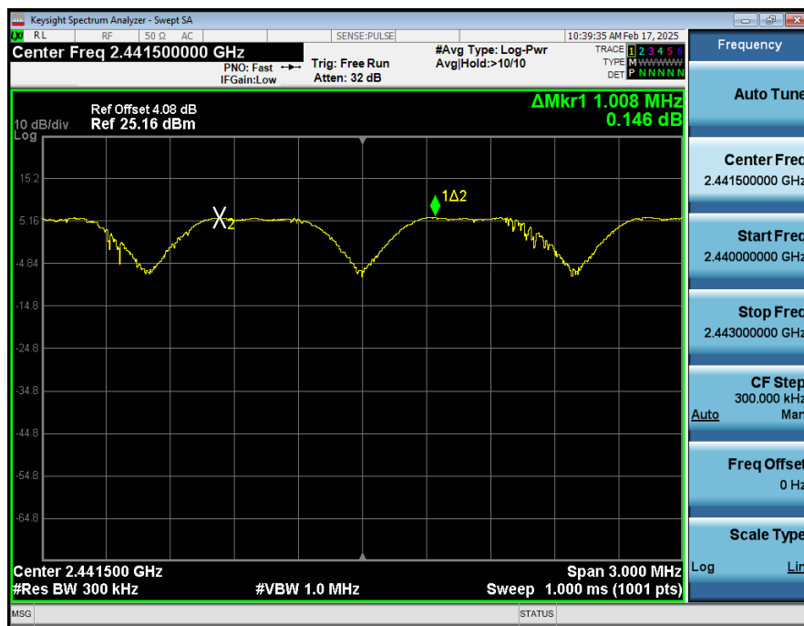
Carrier_Frequencies_Separation_(Hopping)_NVNT_ANT1_1-DH1_Hopping
