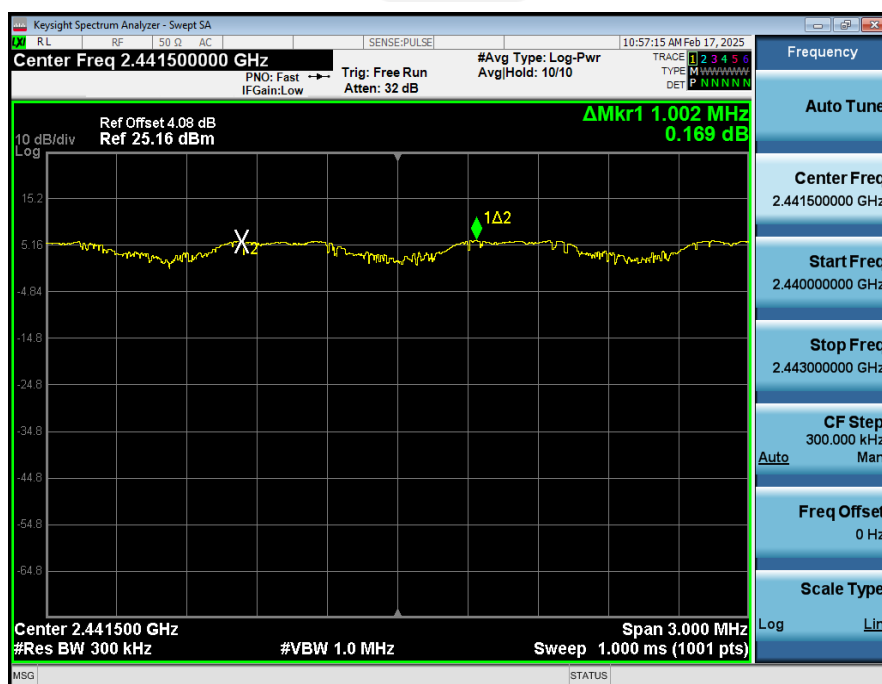
Carrier_Frequencies_Separation_(Hopping)_NVNT_ANT1_2-DH1_Hopping
