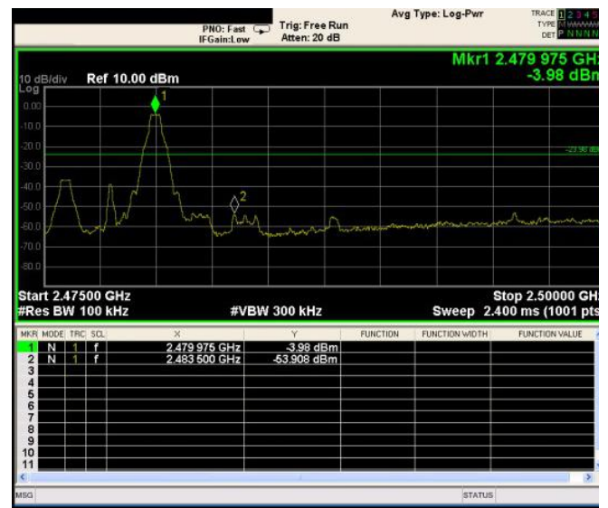
GFSK: Band Edge-High Channel (Hopping Mode)
