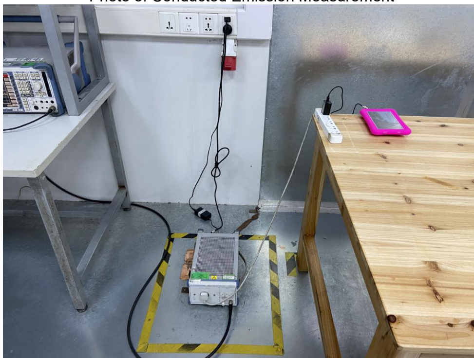
FCC ID: 2AVJH-KIDS08 Photo of Conducted Emission Measurement
