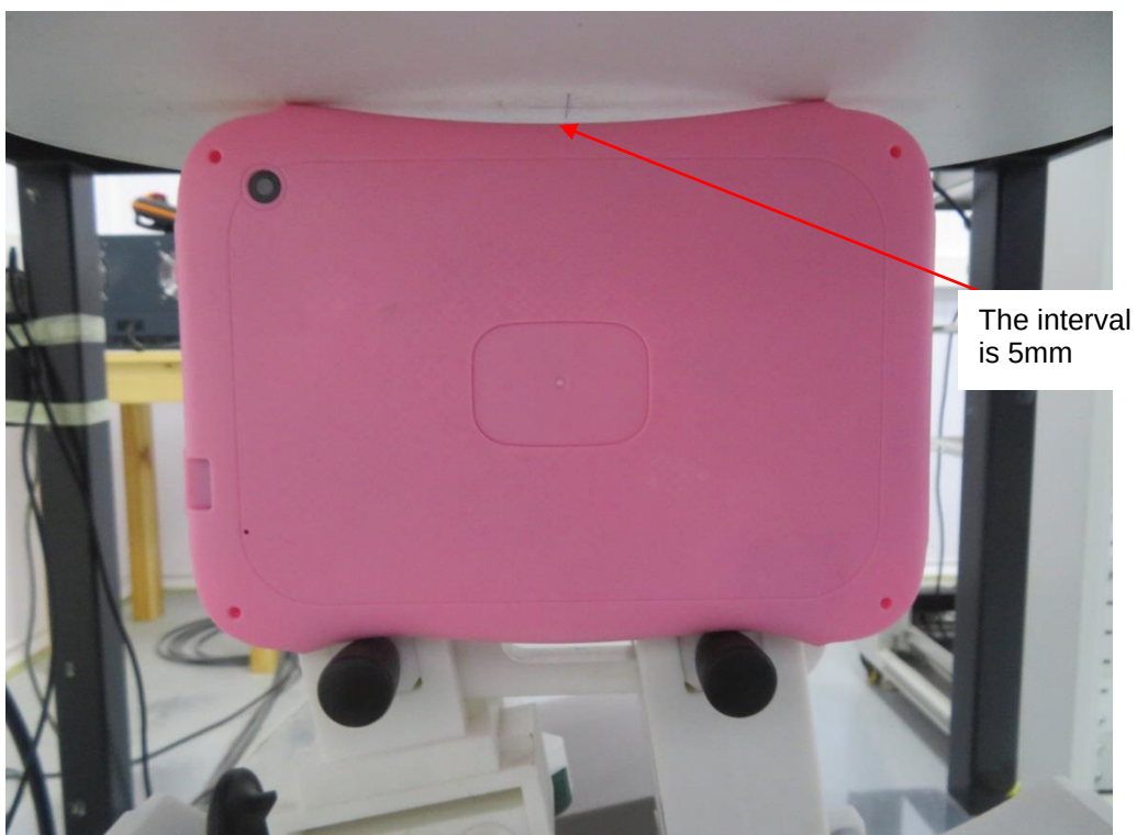
0mm body-worn Top Side Setup Photo
