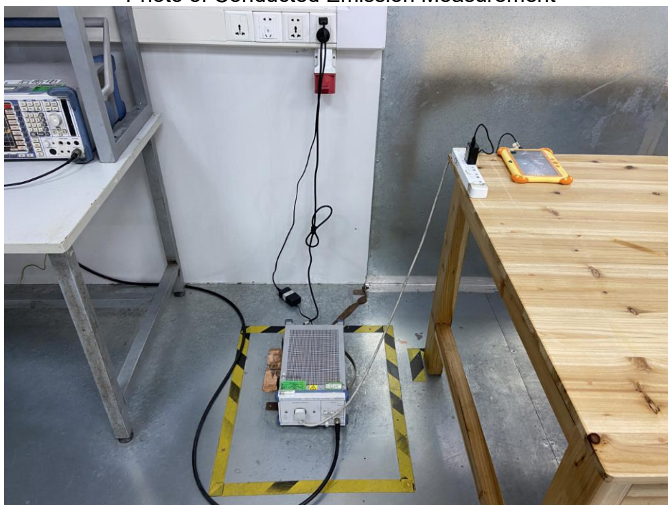
FCC ID: 2AVJH-V7 Photo of Conducted Emission Measurement
