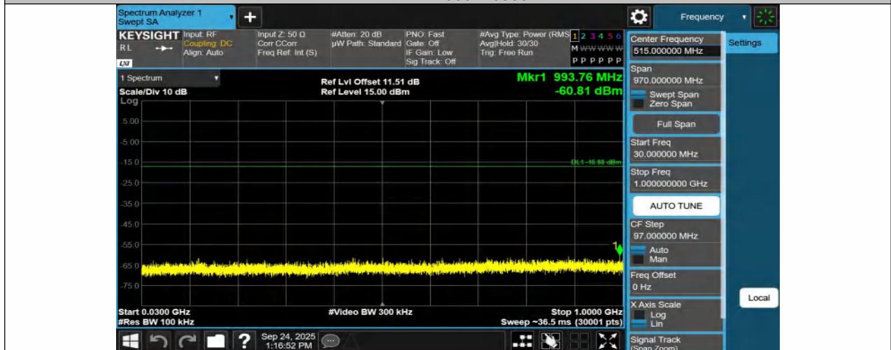
11B-Ant1-2437-30~1000-PASS
