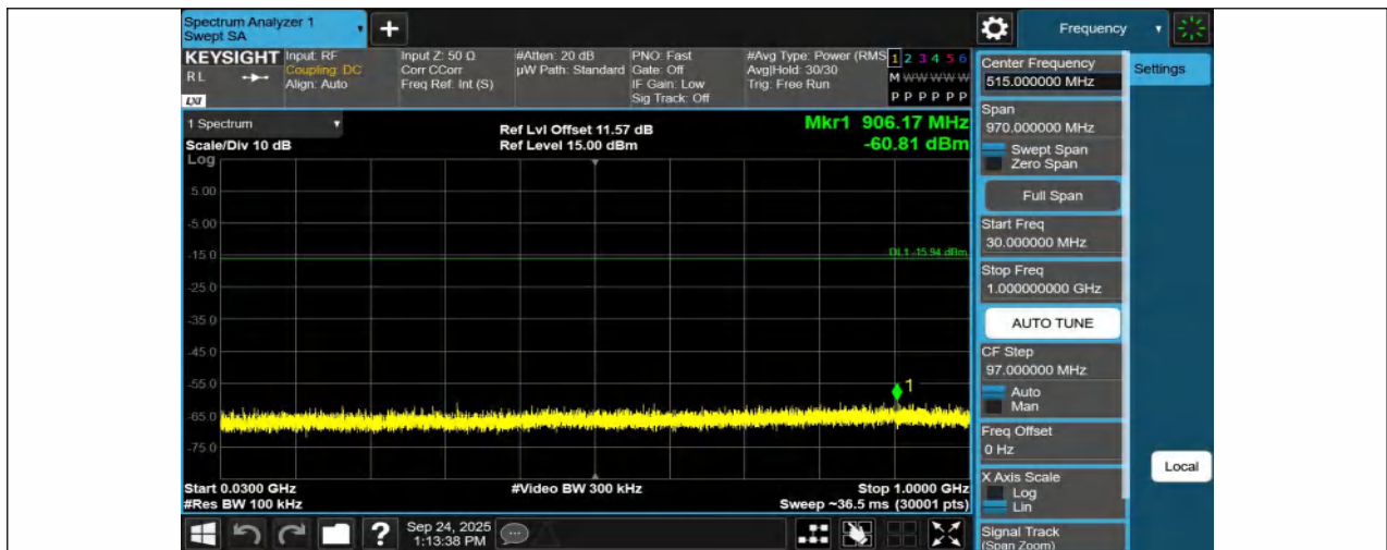
11B-Ant1-2412-30~1000-PASS
