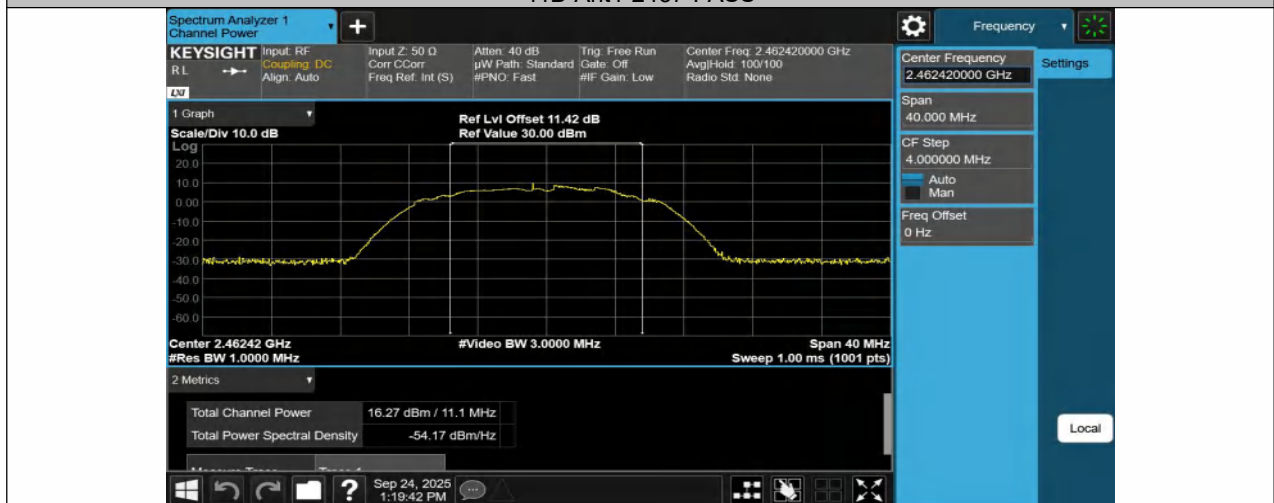
11B-Ant1-2462-PASS
