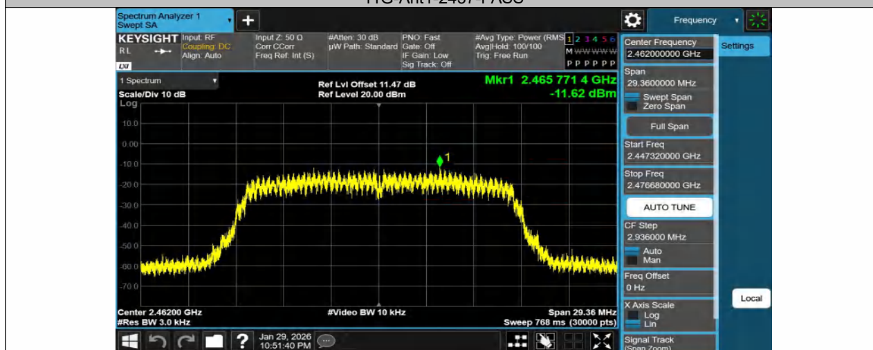
11G-Ant1-2462-PASS
