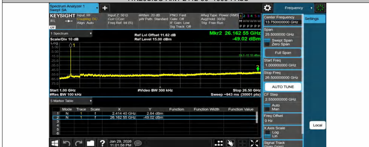
11N20SISO-Ant1-2412-1000~26500-PASS
