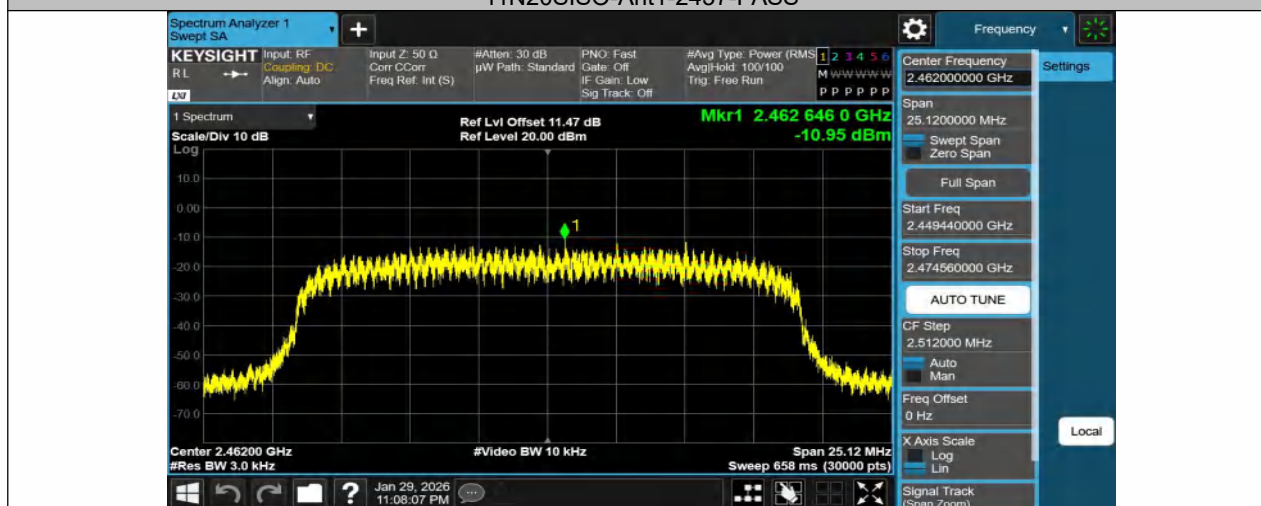
11N20SISO-Ant1-2462-PASS
