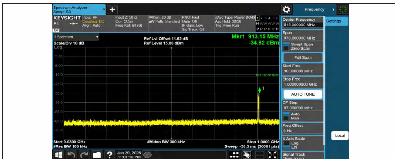
11N20SISO-Ant1-2412-30~1000-PASS
