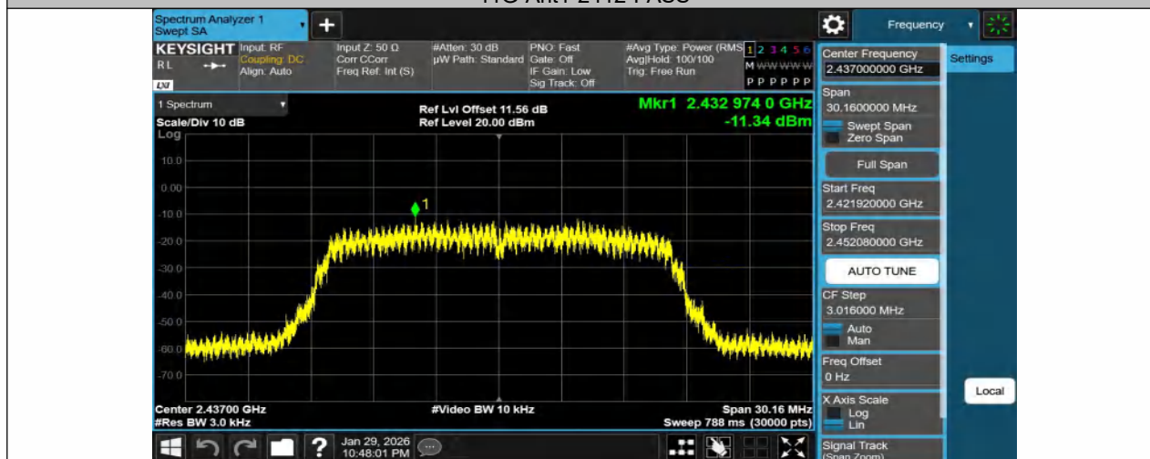
11G-Ant1-2437-PASS
