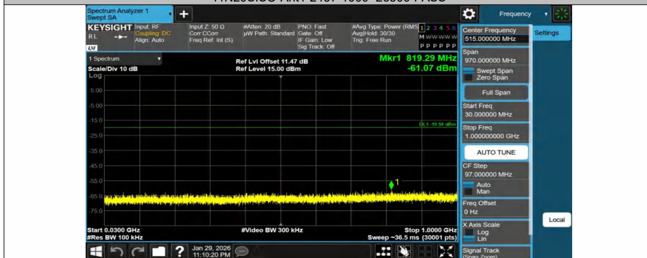
11N20SISO-Ant1-2462-30~1000-PASS
