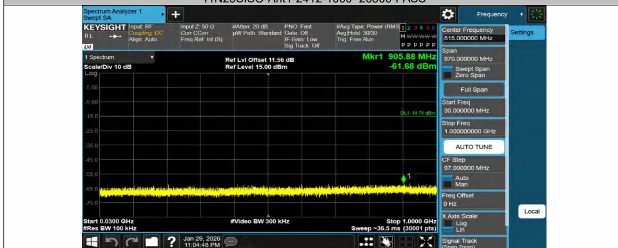
11N20SISO-Ant1-2437-30~1000-PASS
