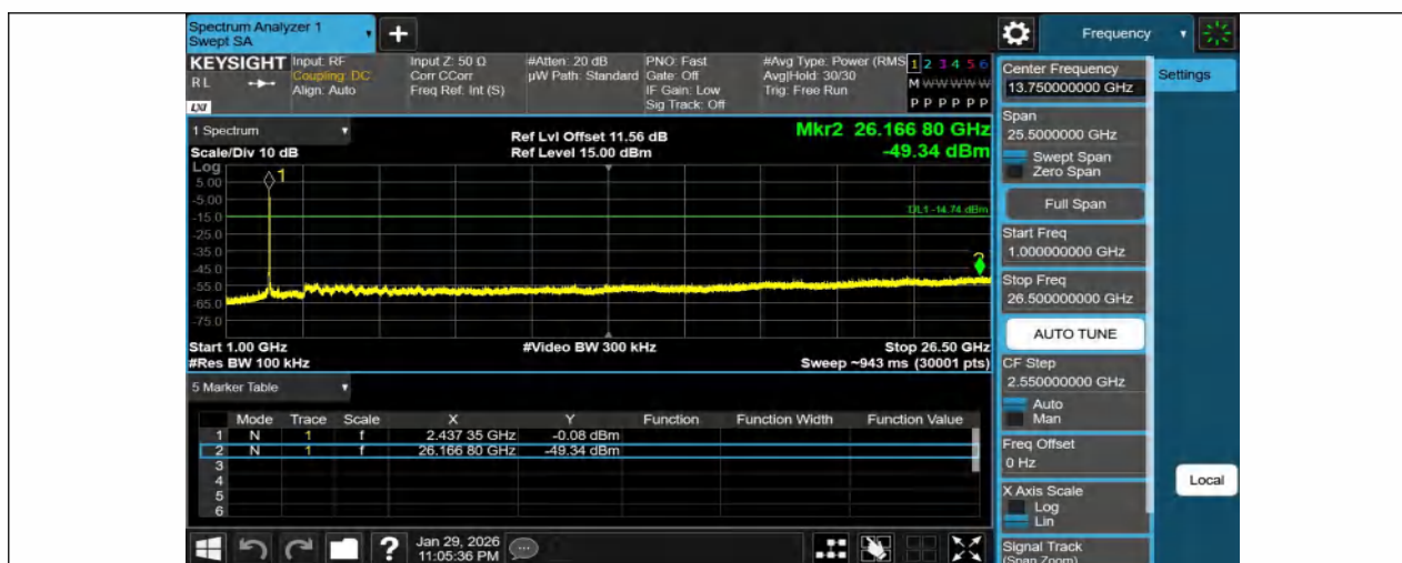
11N20SISO-Ant1-2437-1000~26500-PASS
