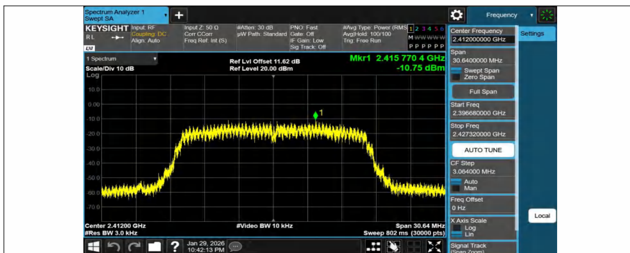
11G-Ant1-2412-PASS
