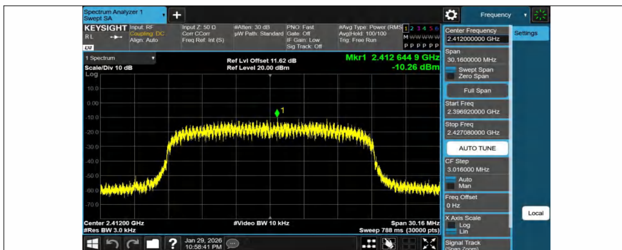
11N20SISO-Ant1-2412-PASS
