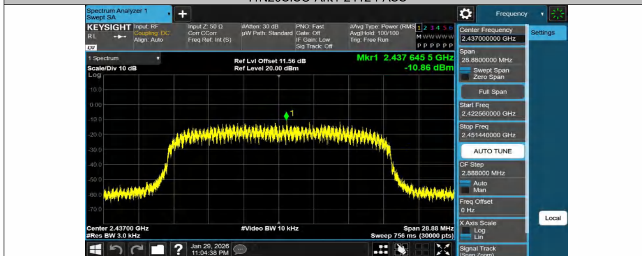
11N20SISO-Ant1-2437-PASS
