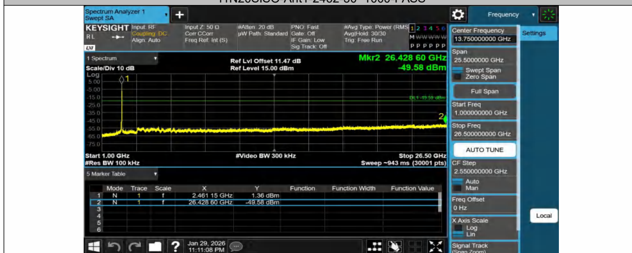
11N20SISO-Ant1-2462-1000~26500-PASS
