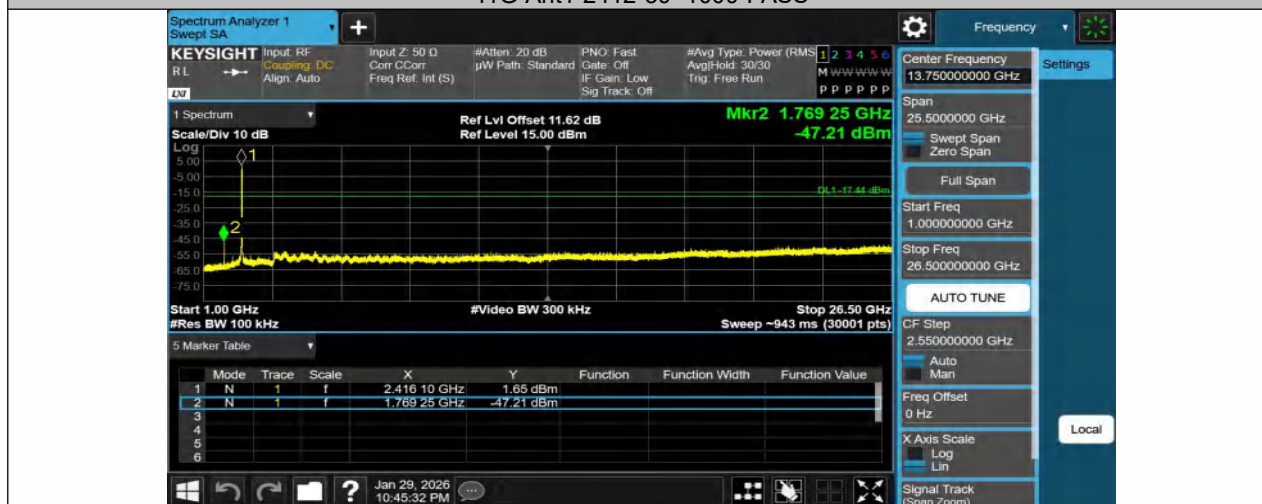
11G-Ant1-2412-1000~26500-PASS
