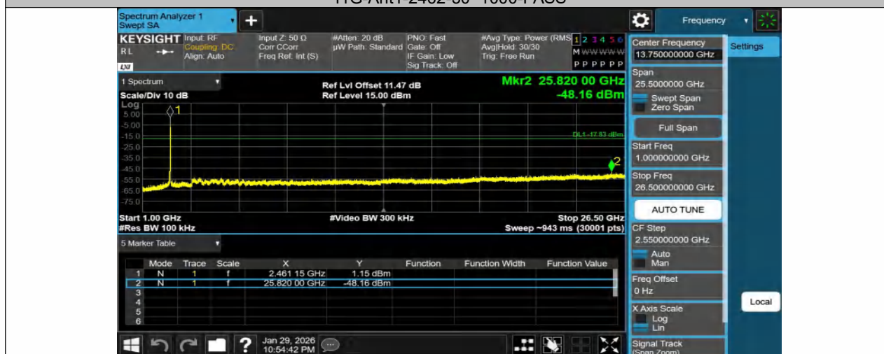
11G-Ant1-2462-1000~26500-PASS
