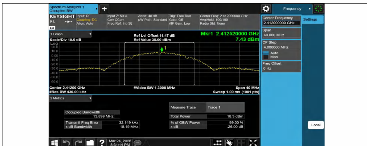
11B-Ant1-2412
