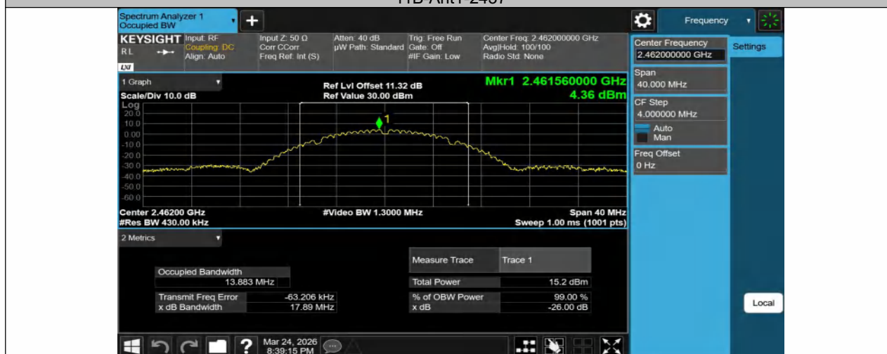
11B-Ant1-2462
