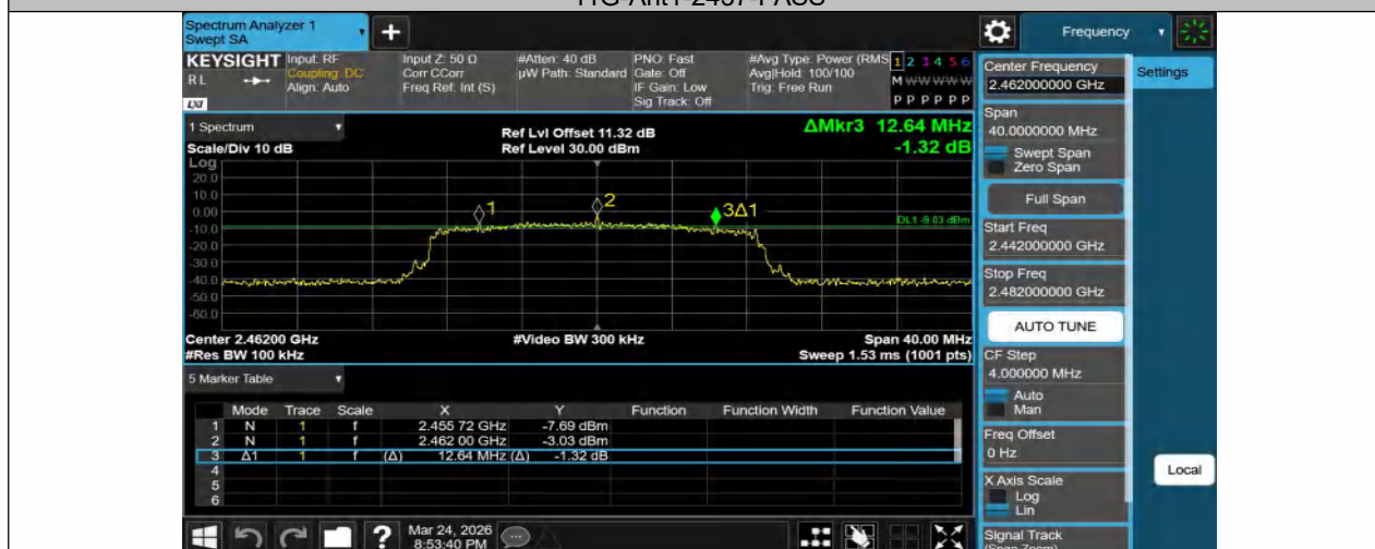
11G-Ant1-2462-PASS
