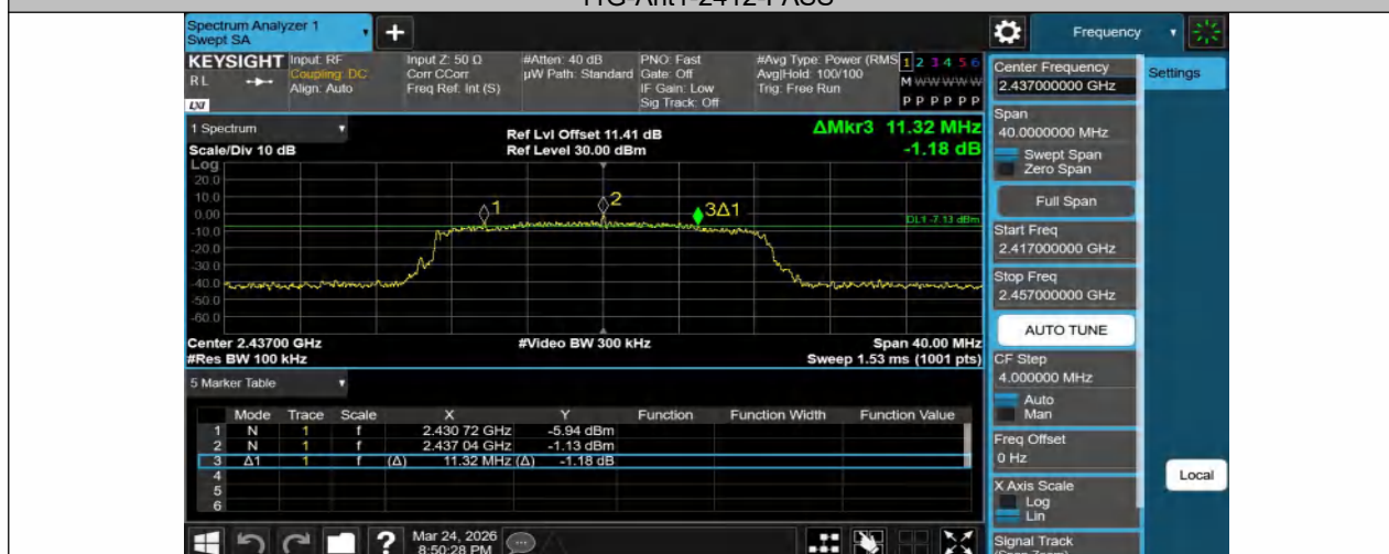
11G-Ant1-2437-PASS
