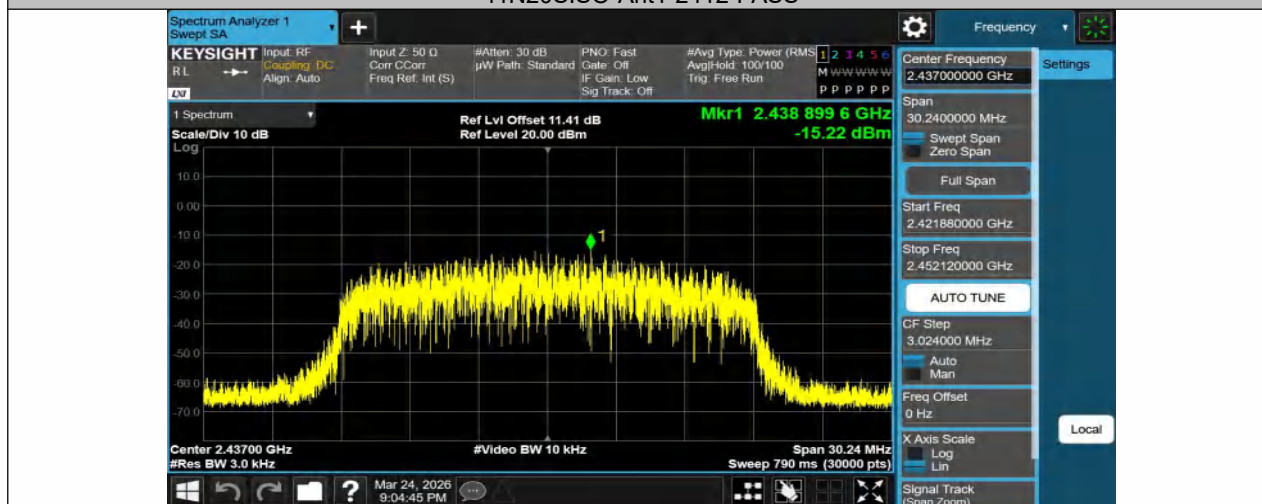
11N20SISO-Ant1-2437-PASS
