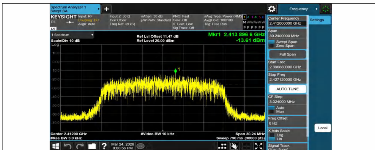
11N20SISO-Ant1-2412-PASS
