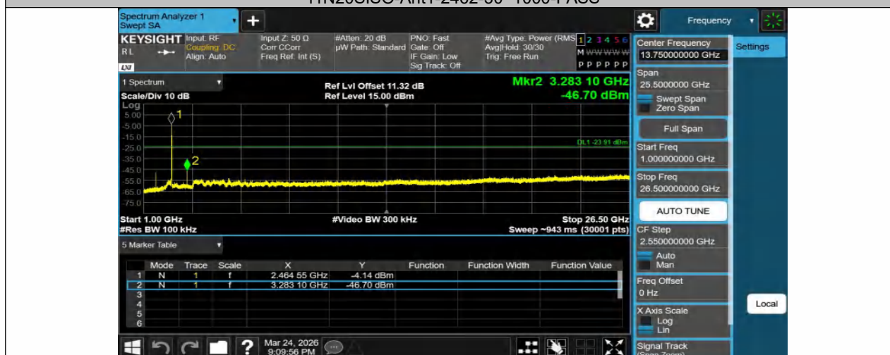
11N20SISO-Ant1-2462-1000~26500-PASS
