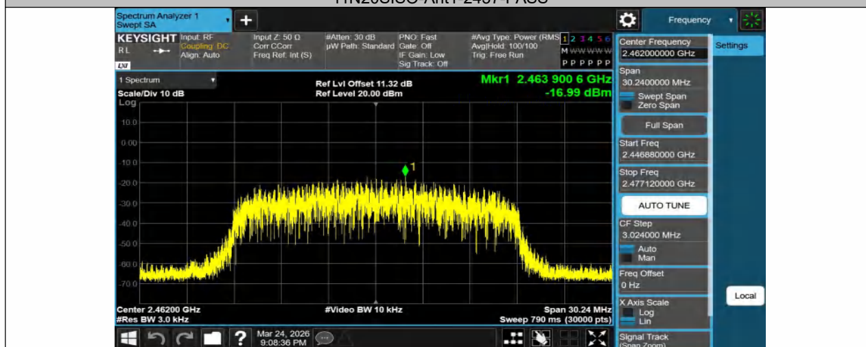
11N20SISO-Ant1-2462-PASS
