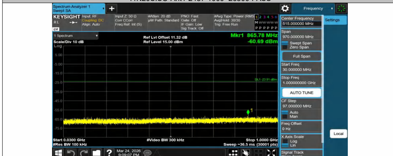
11N20SISO-Ant1-2462-30~1000-PASS
