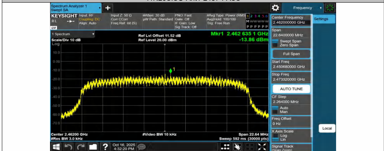
11N20SISO-Ant1-2462-PASS
