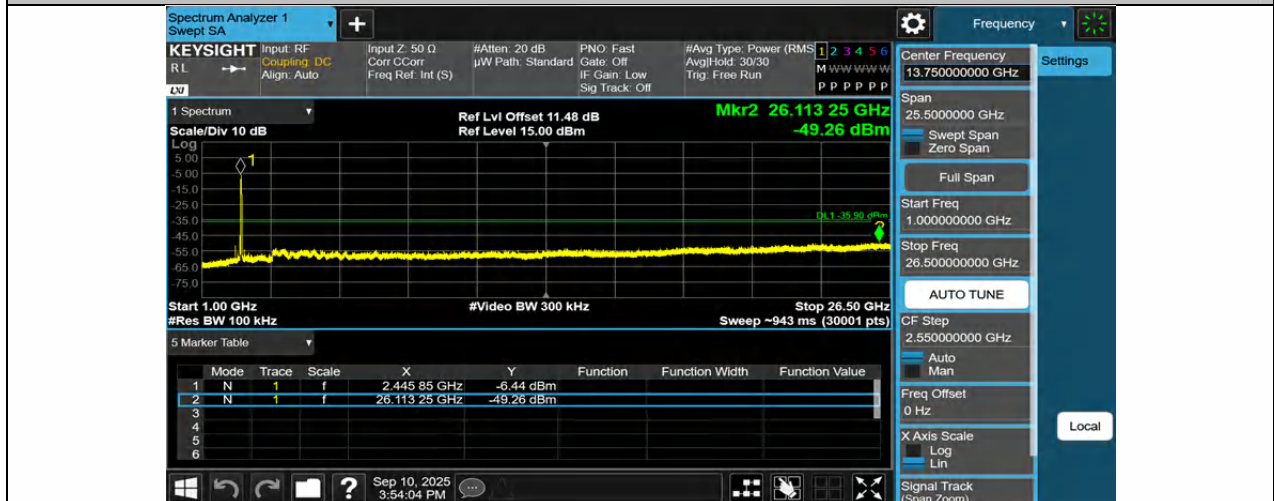
11N40SISO-Ant1-2452-1000~26500-PASS
