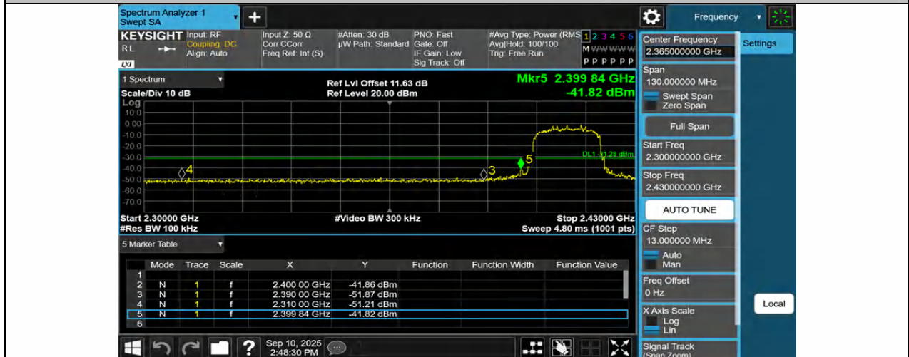
11G-Ant1-2412-PASS
