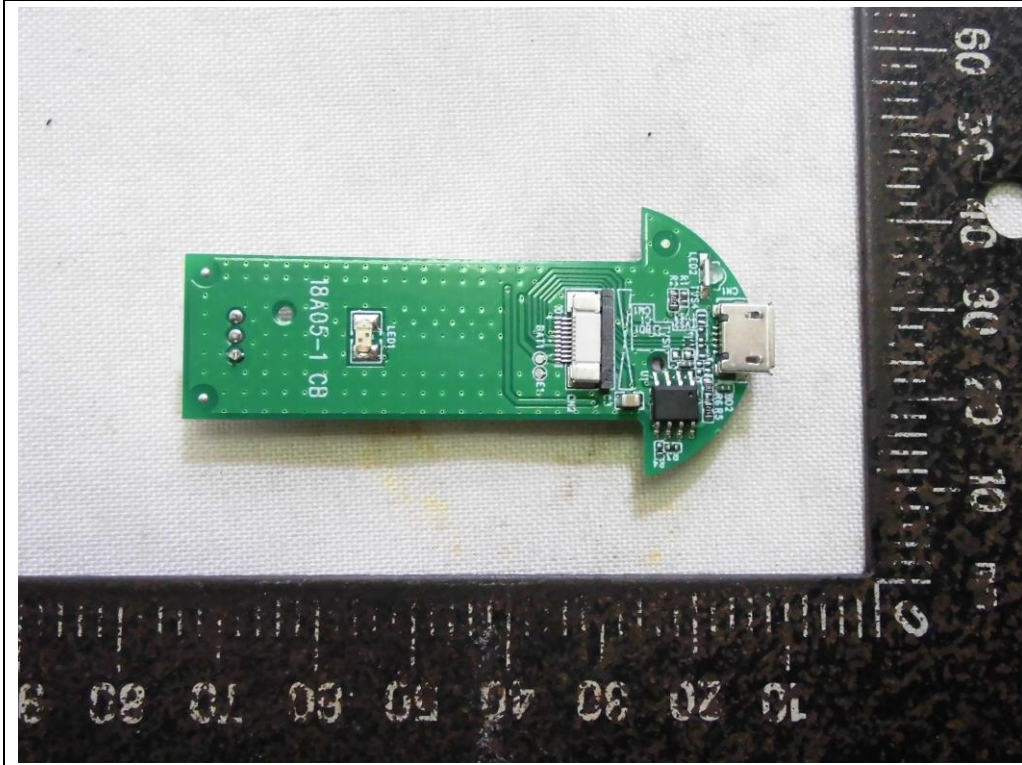
02. Front view of PCB 01
