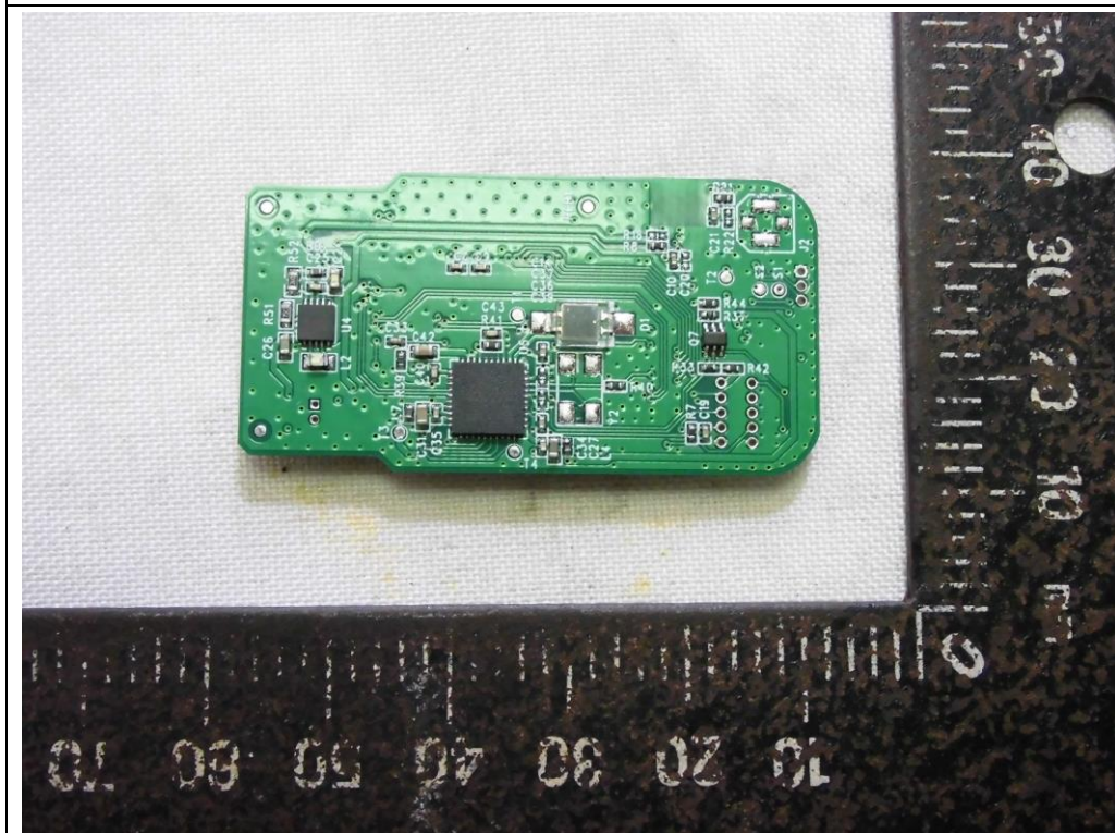
05. Rear view of PCB 02
