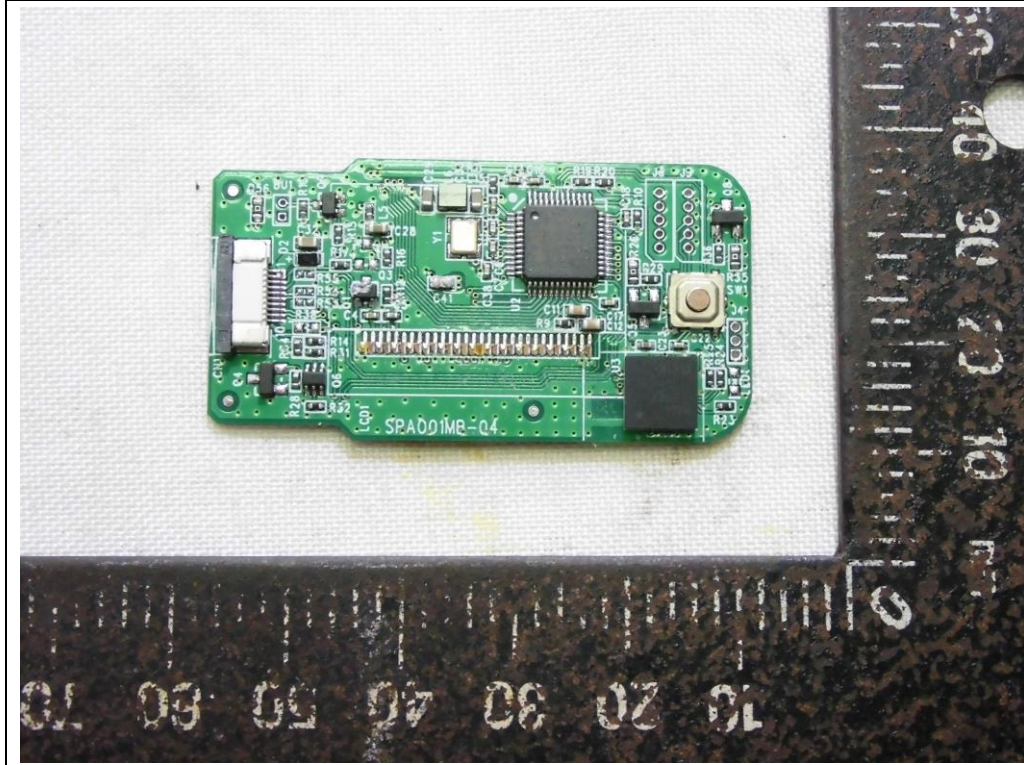
04. Front view of PCB 02
