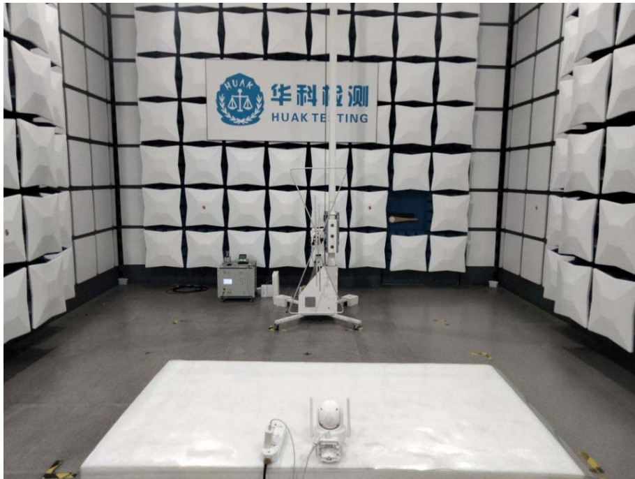
Model: BF-A50G Radiated Emissions
