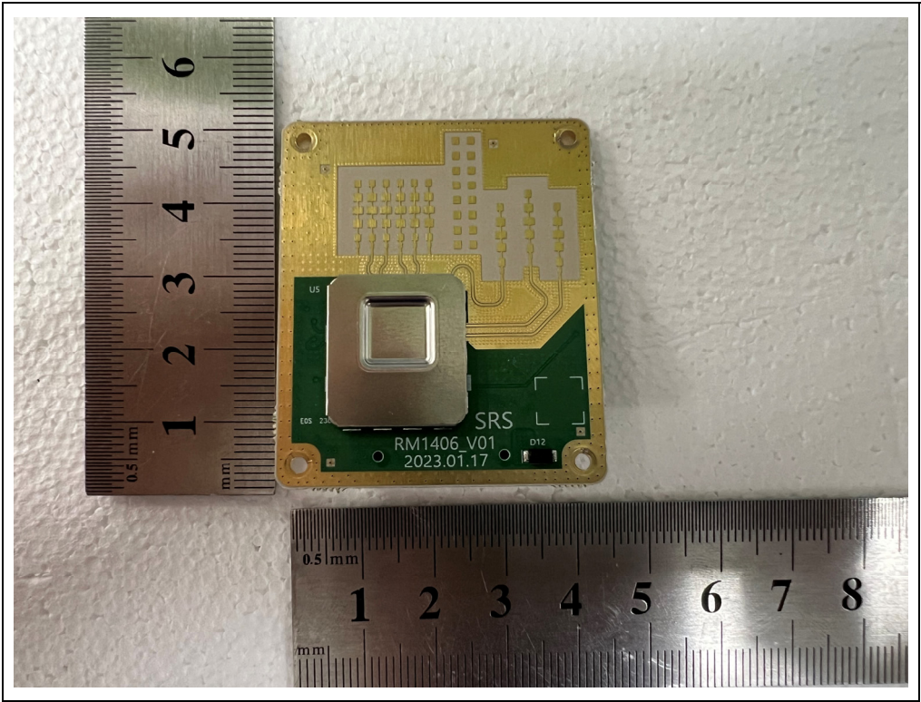
<Module #1>
