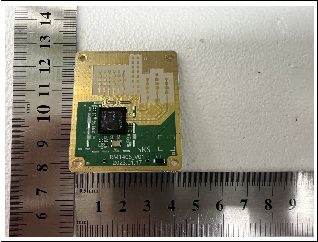
<Module #1>
