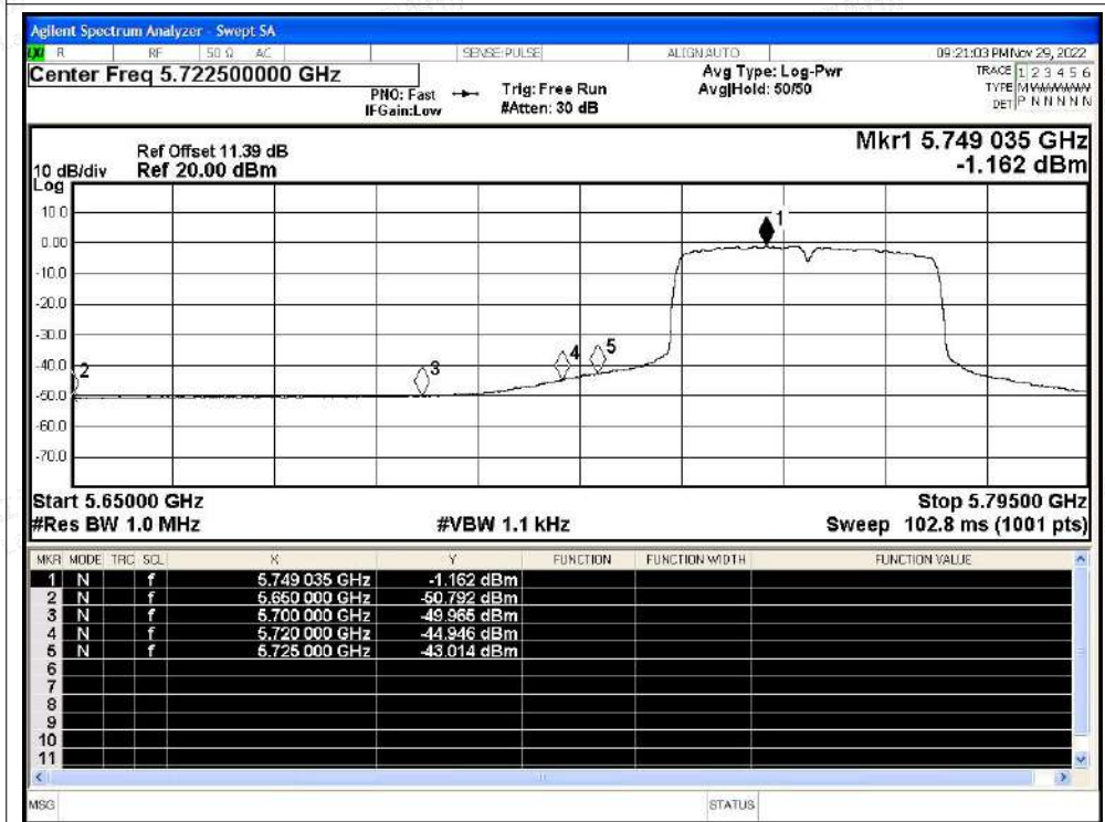
Restrict Band NVNT n40 5755MHz Average
