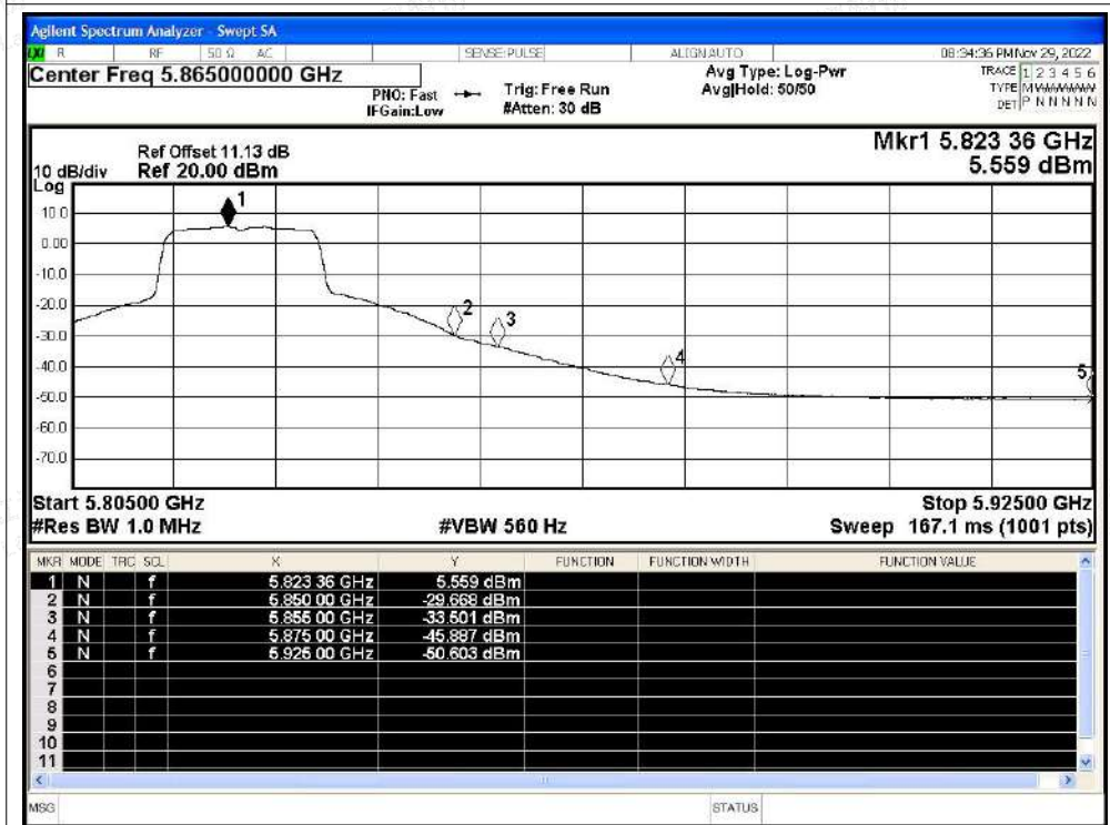
Restrict Band NVNT n20 5825MHz Average
