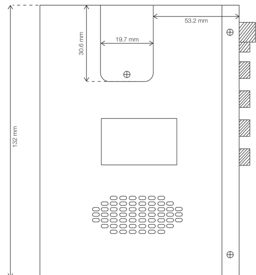
Figure 5. QUARTZ-ONYX left view
