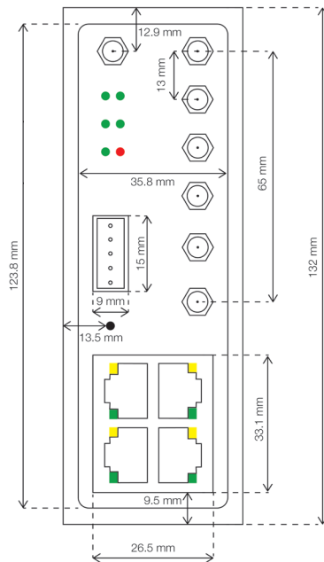
Figure 4. QUARTZ-ONYX top view
