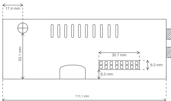
Figure 4. QUARTZ-ONYX top view
