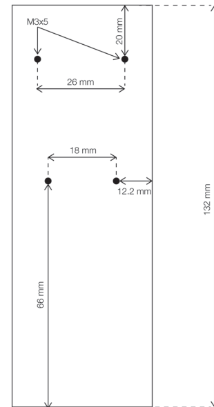
Figure 3. QUARTZ-ONYX rear view
