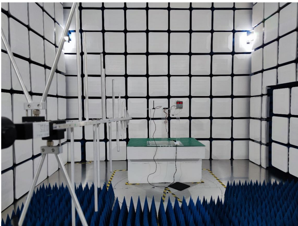
30MHz-1GHz-RF
