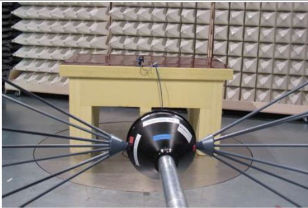
Radiated setup 2
