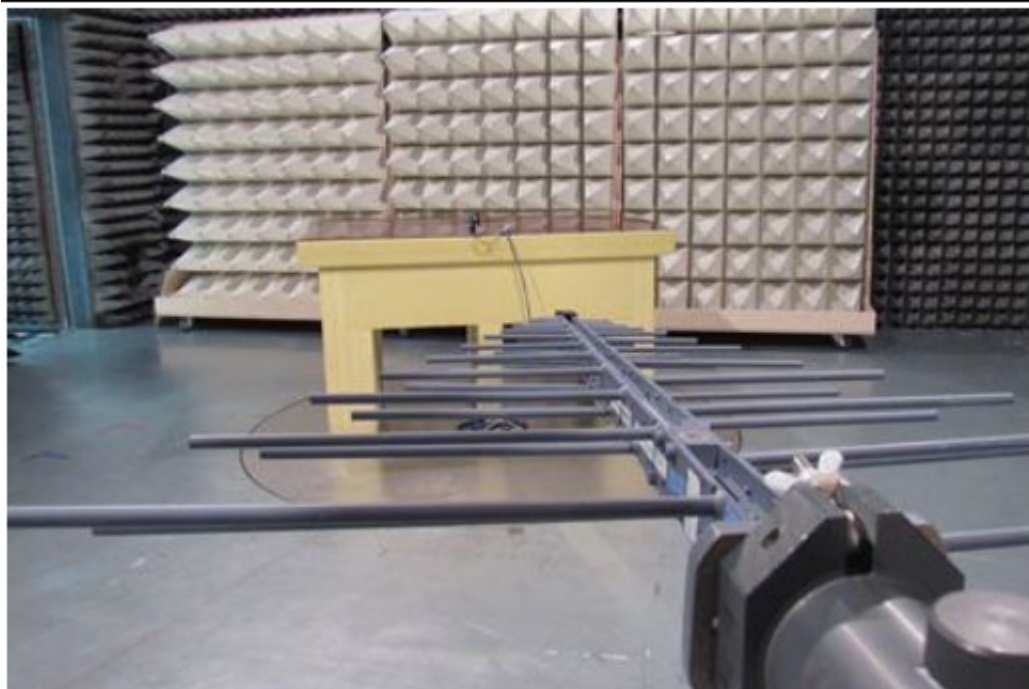
Radiated setup 2
