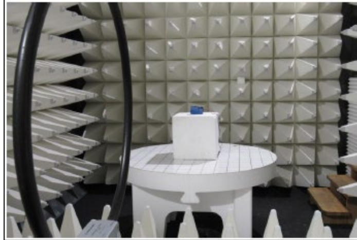
Radiated setup 1
