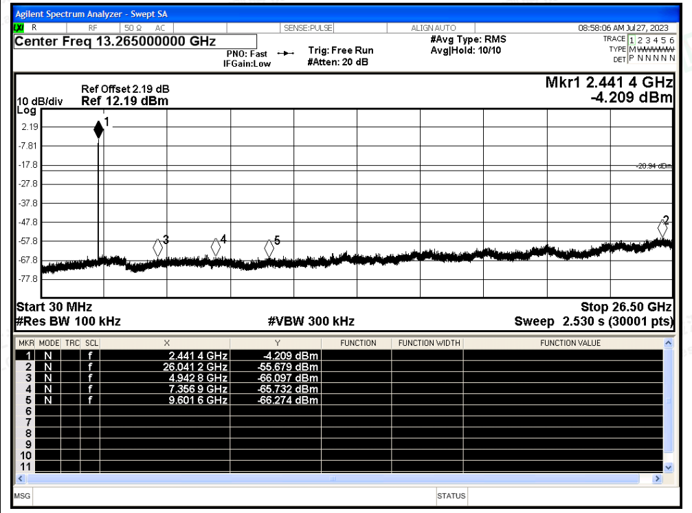
Tx. Spurious NVNT 2-DH5 2441MHz Ant Emission
